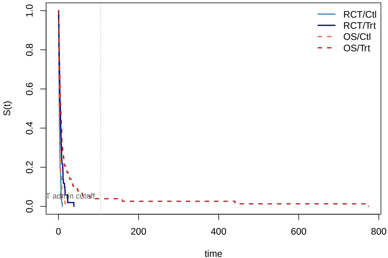
Kaplan-Meier by source and arm
