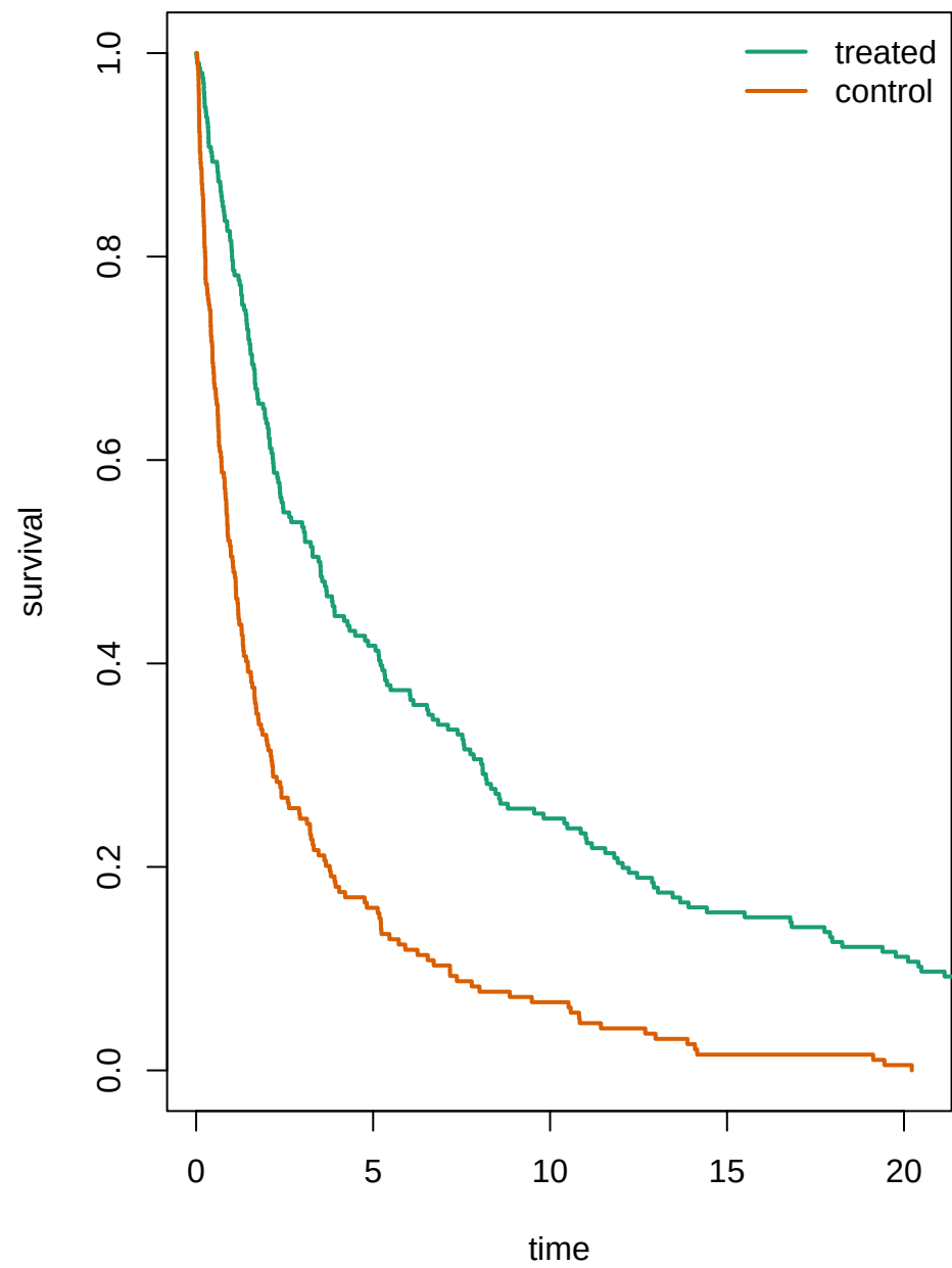
Kaplan-Meier: RWD (interval-censored, approx.)
