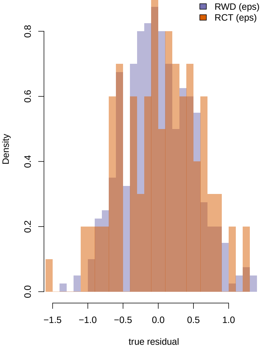
Source residuals (heterogeneous) RCT lognormal / RWD Weibull
