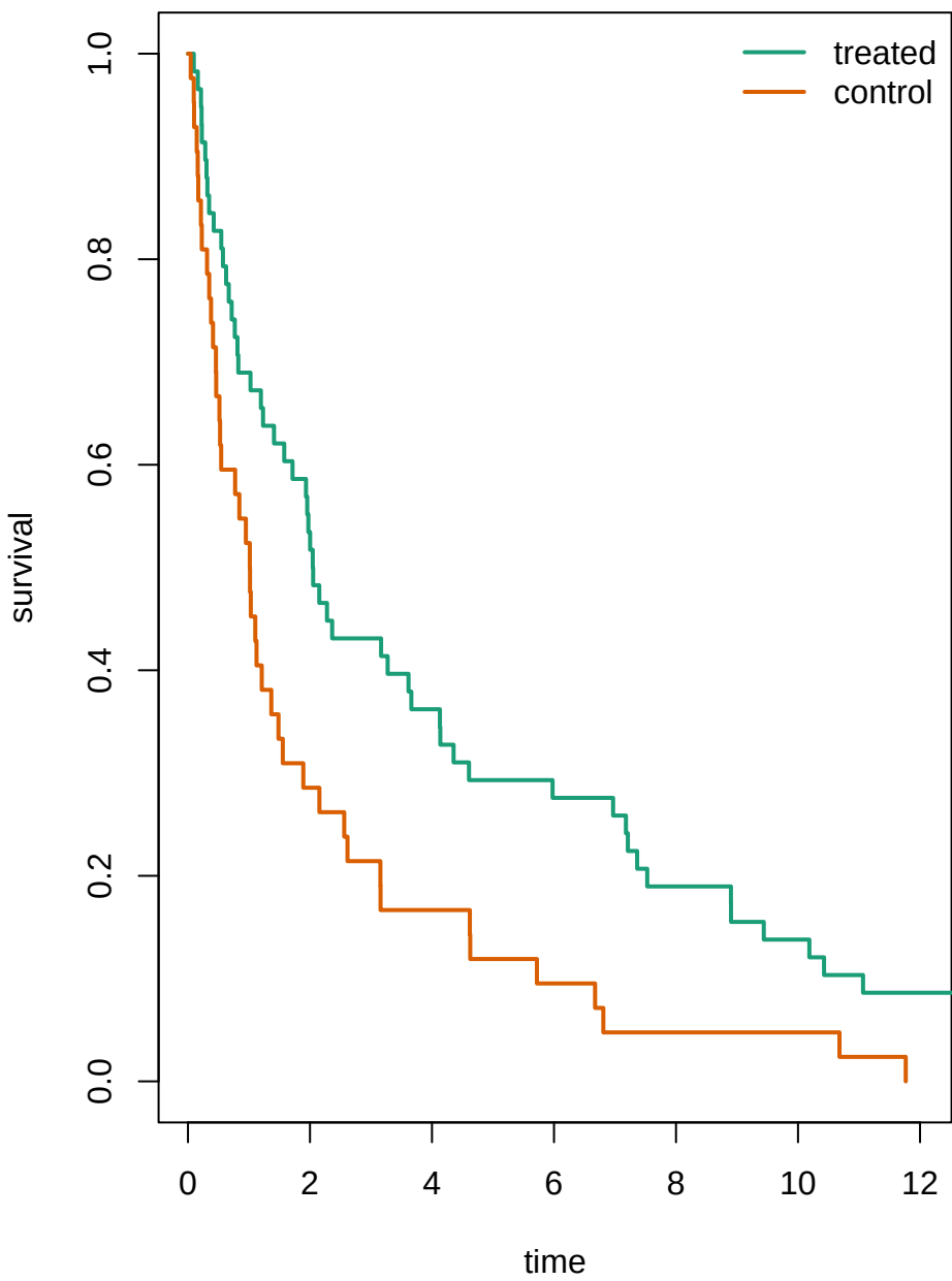
Kaplan-Meier: RCT (right-censored)
