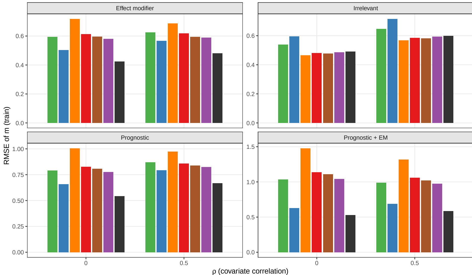
Prediction accuracy – training set
