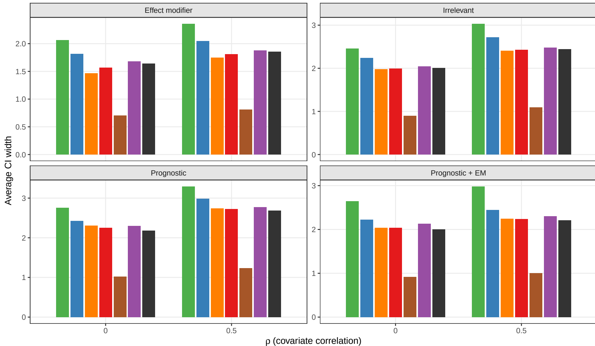
Credible interval width for CATE
