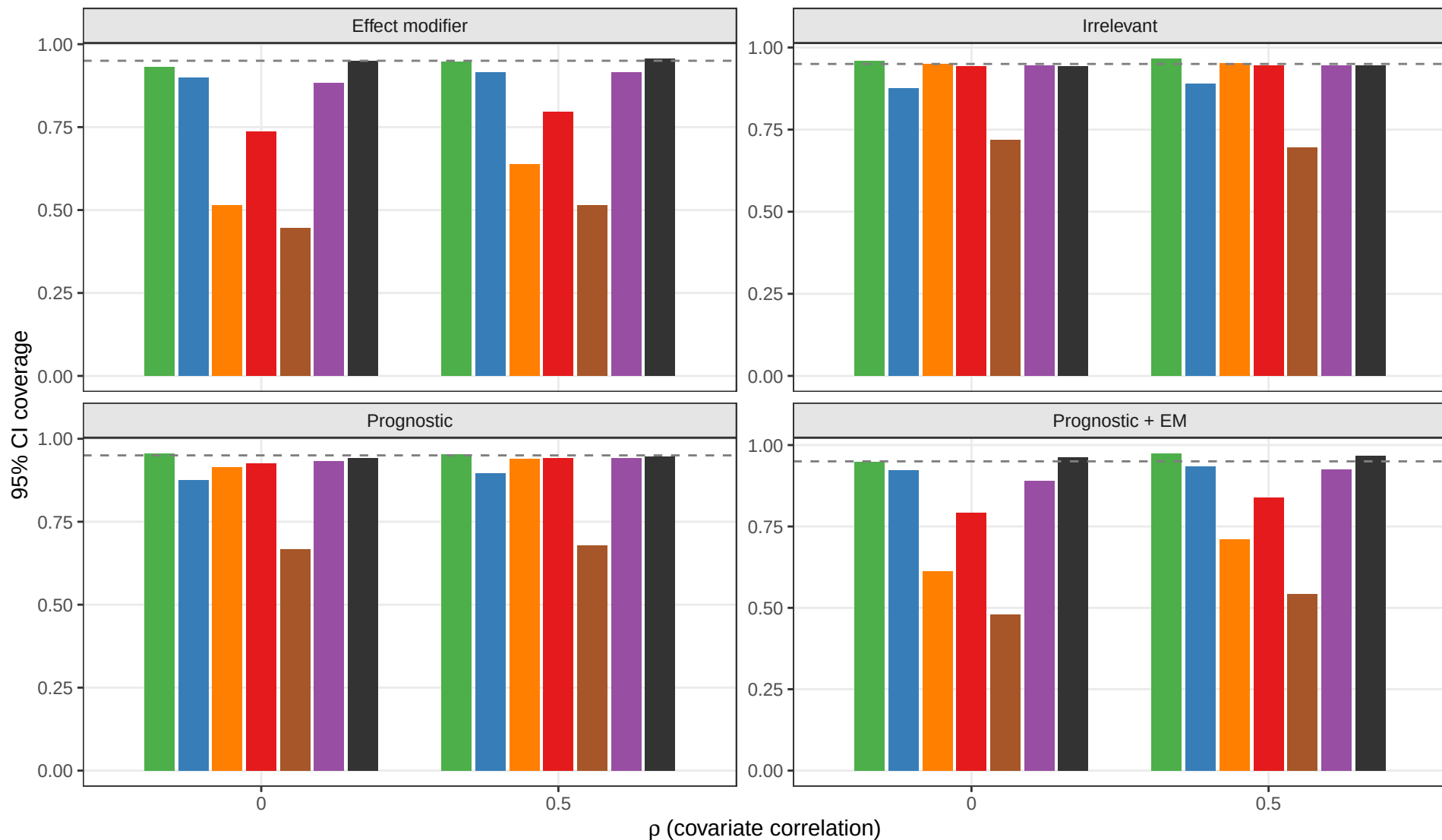
Credible interval coverage for CATE
