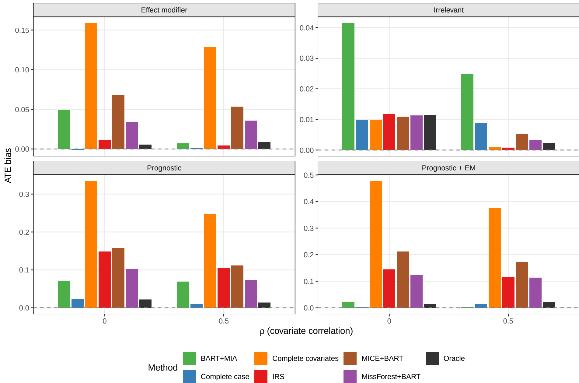
Bias in average treatment effect
