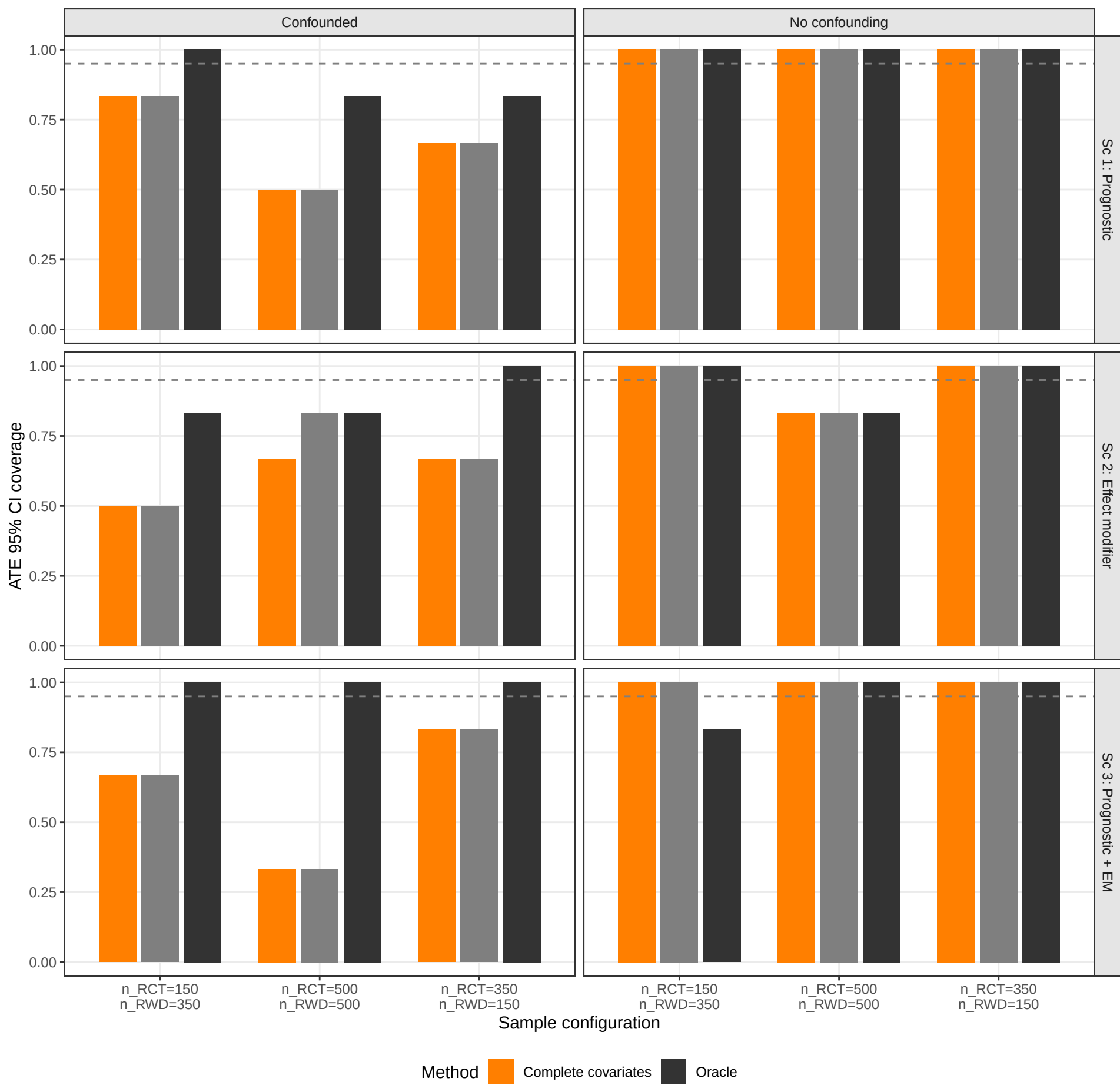
ATE credible interval coverage
