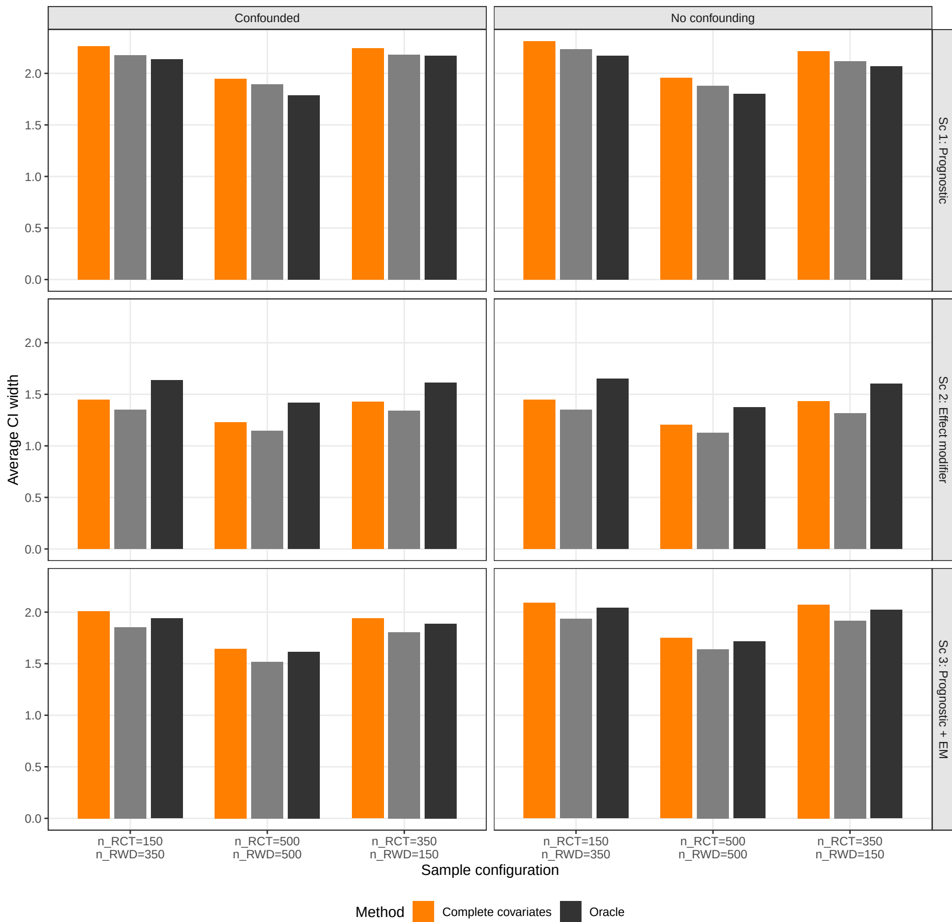
Credible interval width
