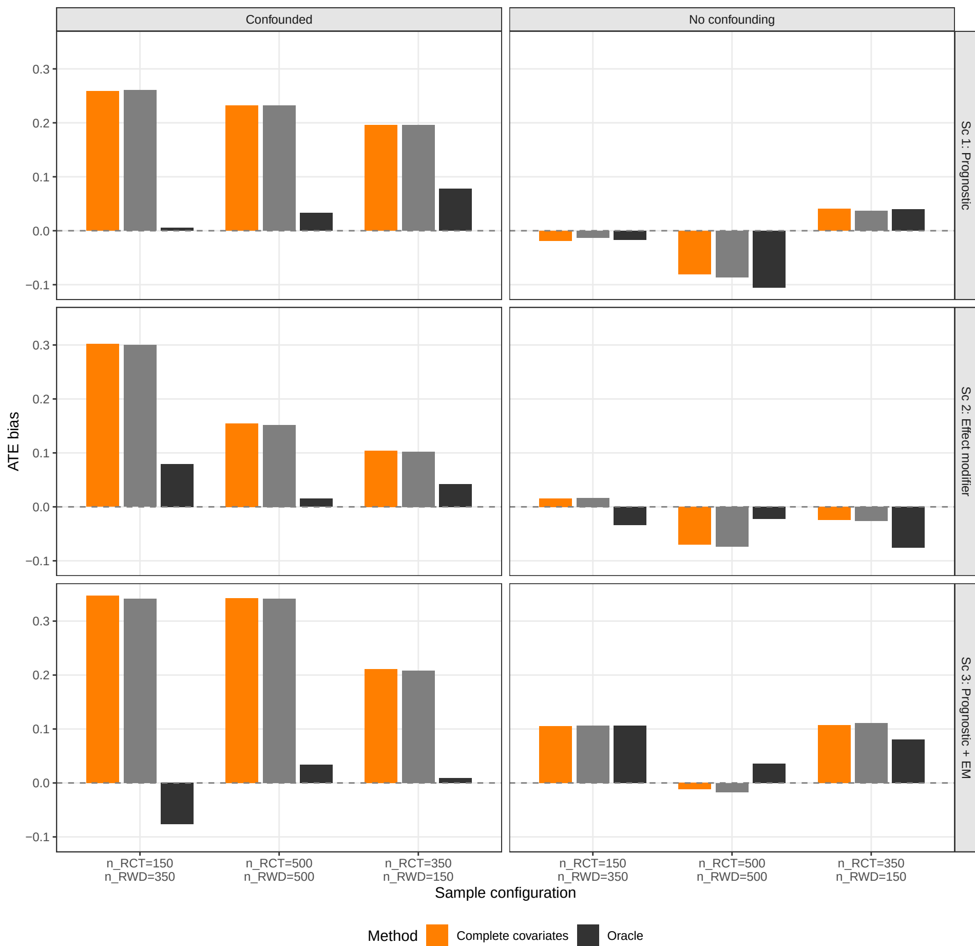
Bias in ATE estimation
