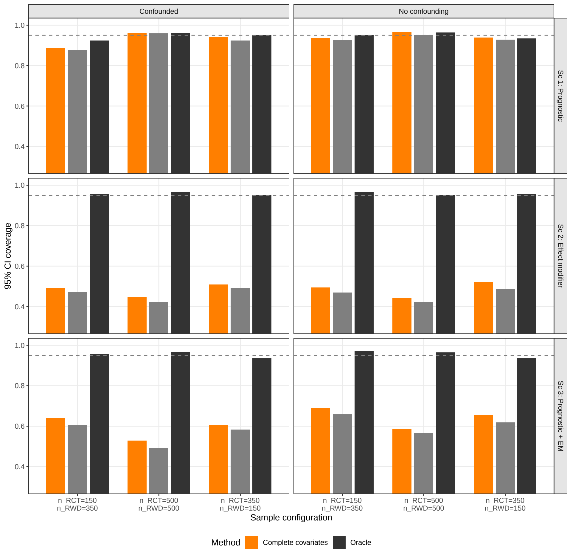
Credible interval coverage
