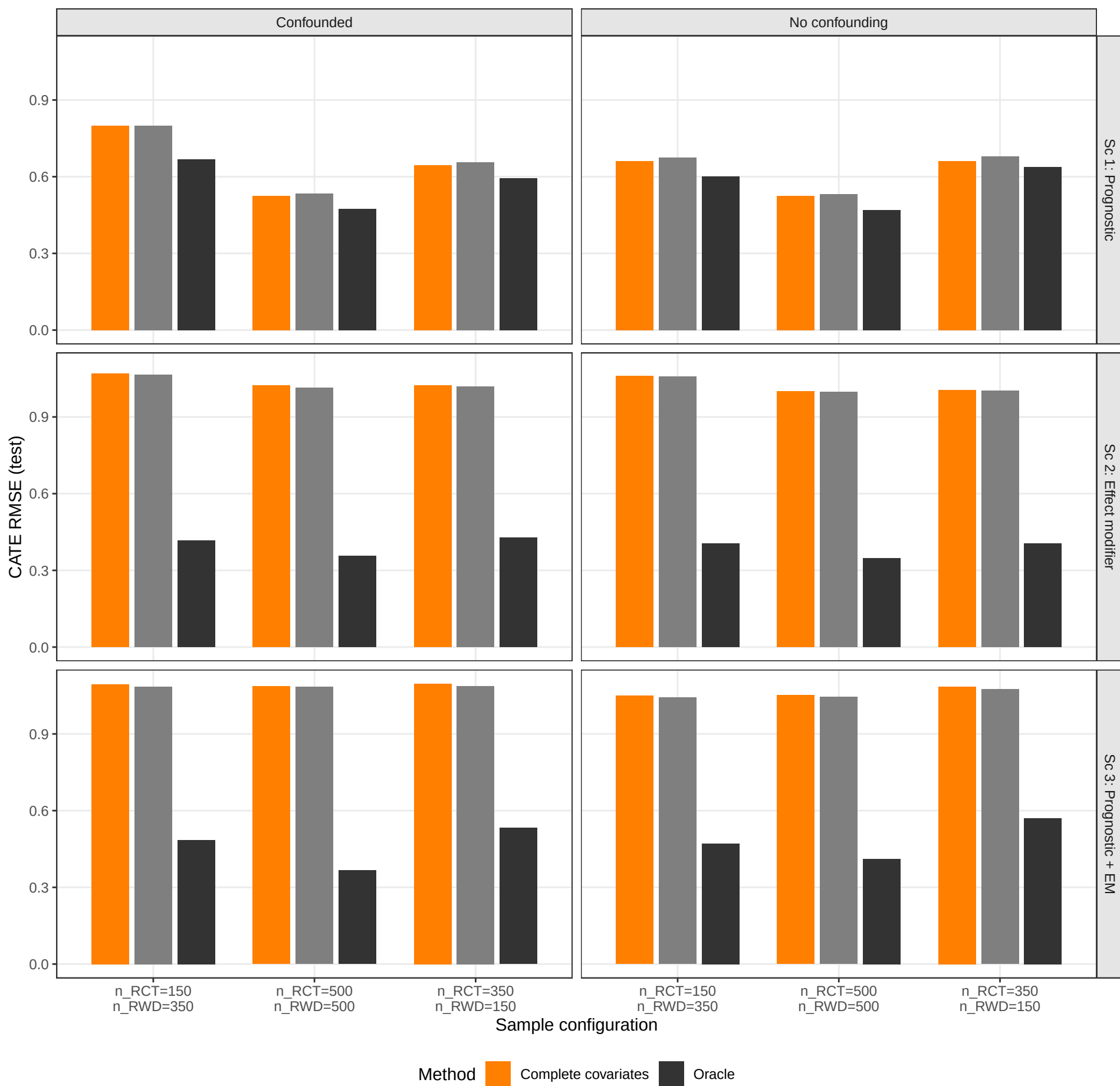
CATE estimation accuracy
