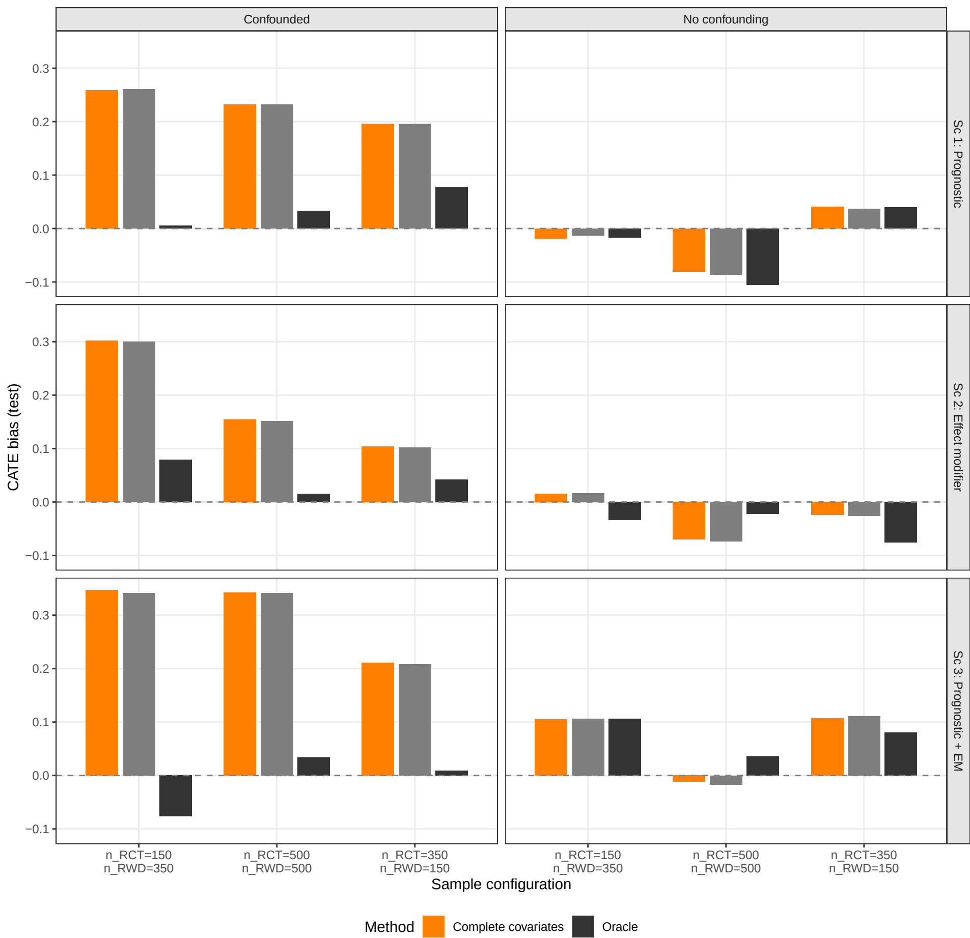
CATE estimation bias
