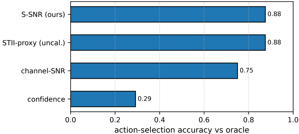
S-SNR vs task-info (STII) and channel proxies
