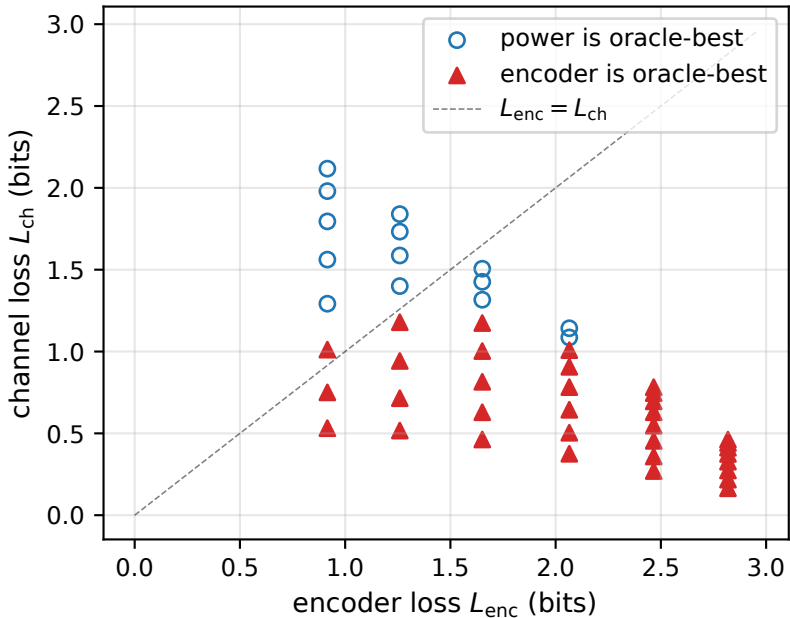
Causal regimes vs. oracle-best action
