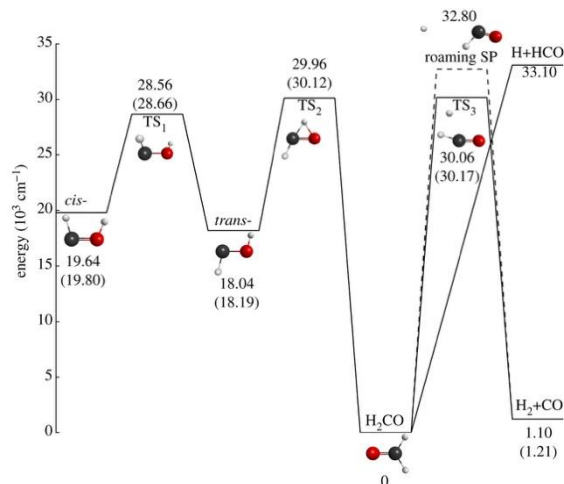
Potential energy surface for \text{H}_2\text{CO}
