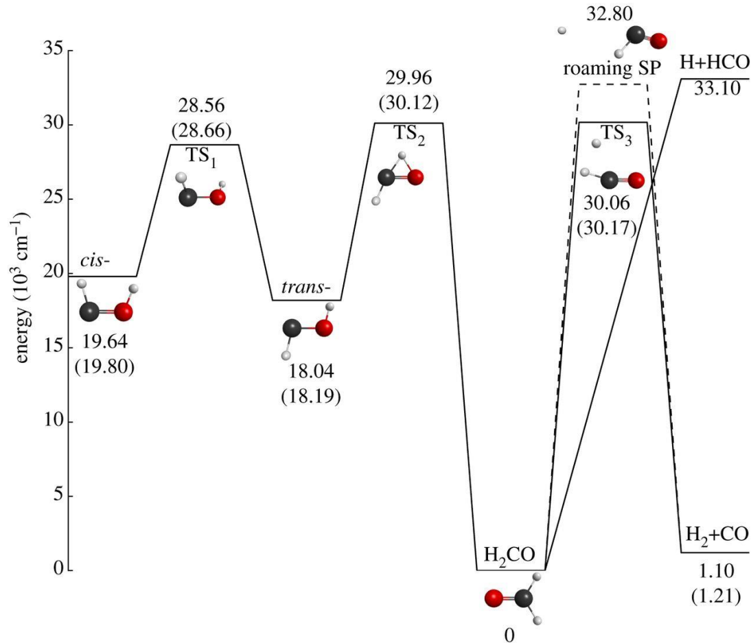
Stationary structures of \text{H}_2\text{CO}
