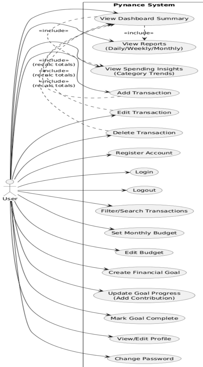
Figure 1: Use Case Diagram for Pynance
