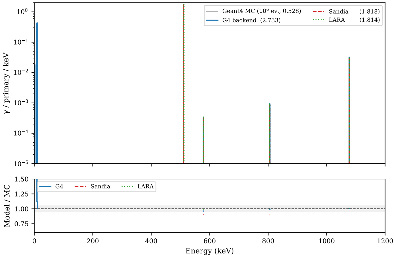
^{68}\text{Ge} secular equilibrium - Ge-68/Ga-68 PET generator (legend values: \gamma /primary totals)
