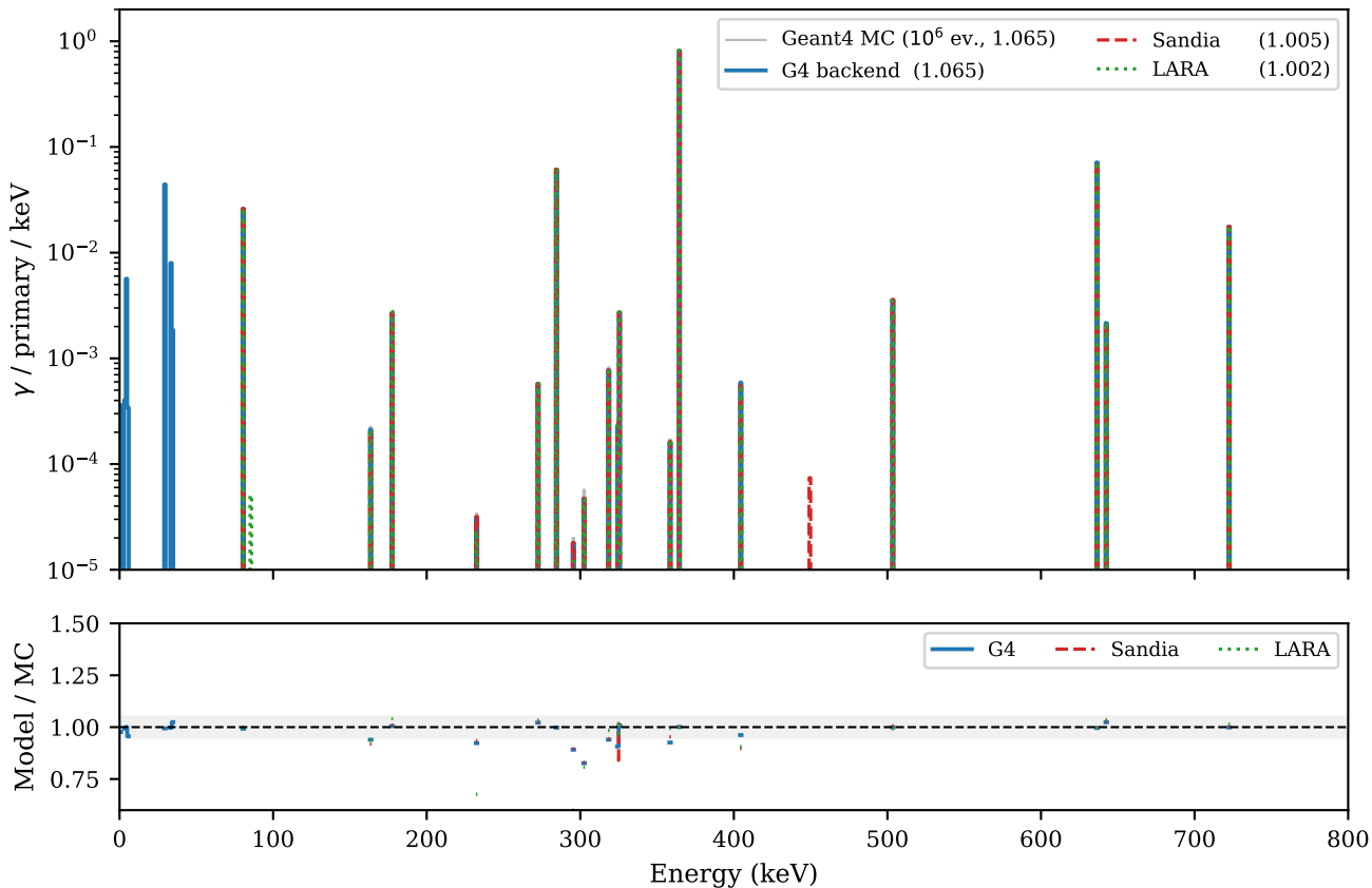
^{131}\text{I} secular equilibrium - I-131 chain (legend values: \gamma /primary totals)
