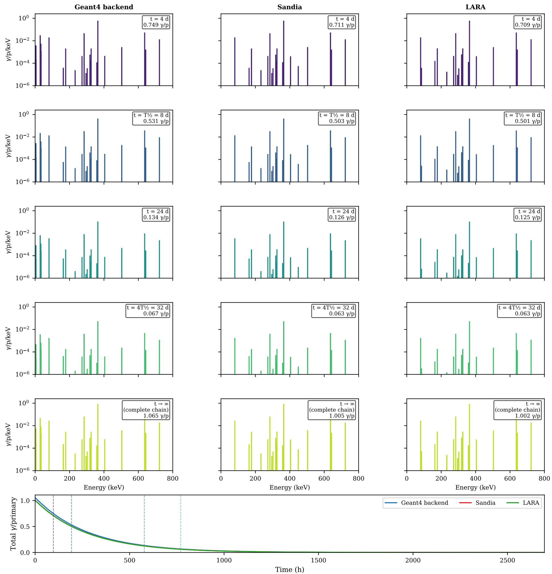
^{131}\text{I} time-dependent spectrum - I-131 chain ( T_{1/2}=8.02 d)
