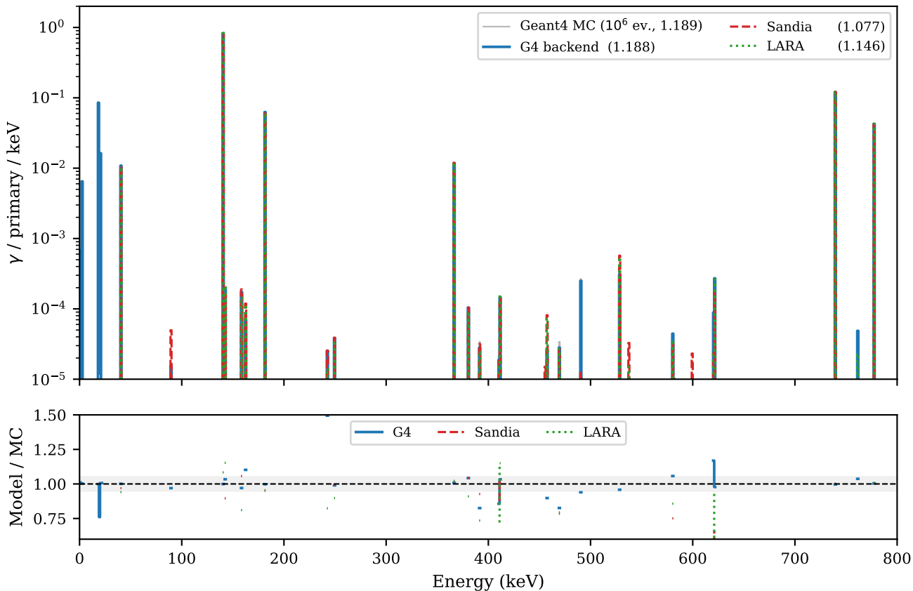
^{99}\text{Mo} secular equilibrium - Mo-99 + Tc-99m chain (legend values: \gamma /primary totals)
