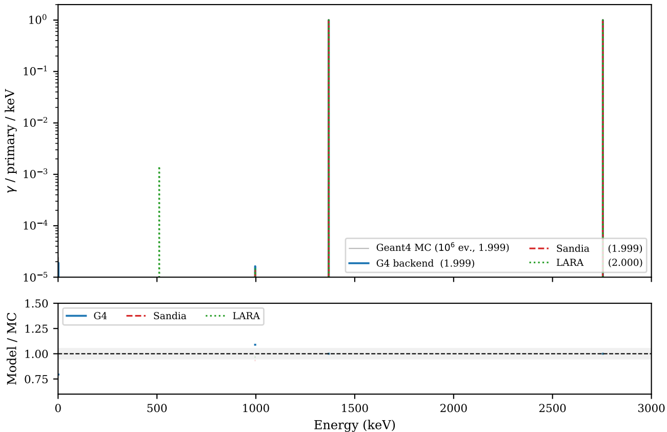
^{24}\text{Na} secular equilibrium - reactor activation (legend values: \gamma /primary totals)
