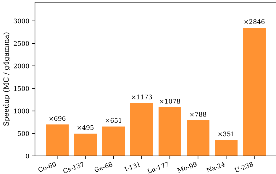
g4gamma speedup over Geant4 MC
