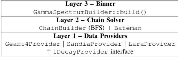
Fig. 1: Three-layer architecture of g4gamma. Each provider exposes a uniform get(IsotopeKey) API returning per-decay photon emissions.
