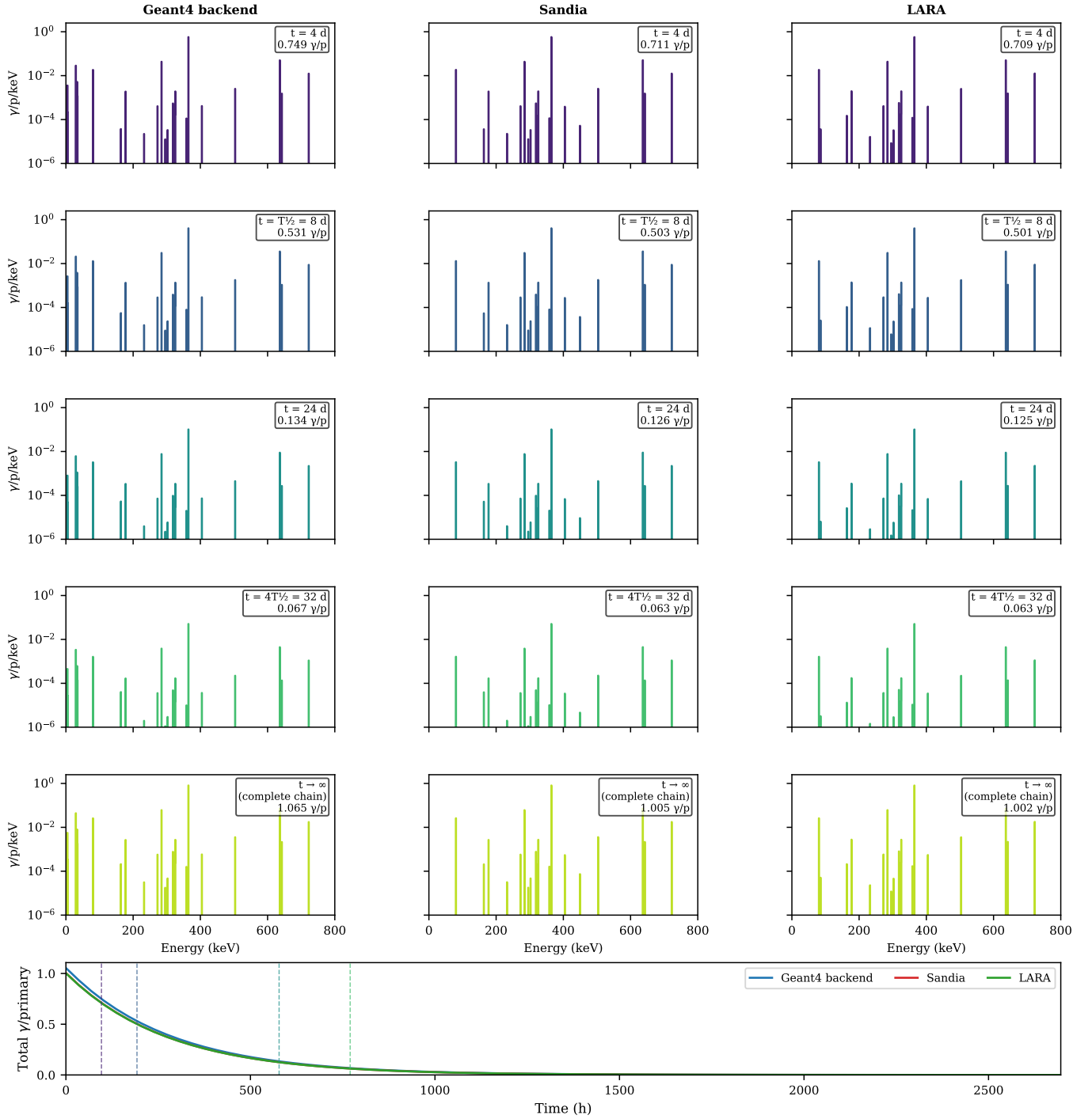
Fig. 20: ^{131}\text{I} time-dependent spectra. Rows: t = 4 d ( T_{1/2}/2 ), T_{1/2} = 8 d, 3T_{1/2} = 24 d, 4T_{1/2} = 32 d, complete chain ( t \rightarrow \infty ). The dominant 364.5 keV line decreases with ^{131}\text{I} 's 8.02 d half-life; at 4T_{1/2} the total activity is \sim 6\% of the initial value. The complete-chain panel is nearly indistinguishable from a fresh source: the only growing daughter, ^{131m}\text{Xe} , has a branching fraction of 1.08% and is in the no-equilibrium regime ( T_{1/2} = 11.8 d > parent 8.02 d), reaching a steady-state activity of only \approx 0.011 per primary—too small to alter the spectral shape visually.
