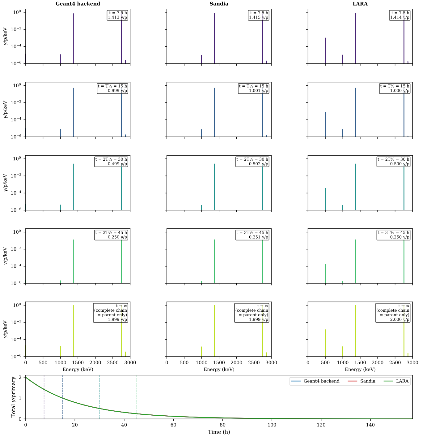
Fig. 18: ^{24}\text{Na} time-dependent spectra. Rows: t = 7.5 h, T_{1/2} = 15 h, 2T_{1/2} = 30 h, 3T_{1/2} = 45 h, complete chain ( t \rightarrow \infty ). The simple \beta^- chain ( ^{24}\text{Na} \rightarrow ^{24}\text{Mg} stable) shows monotonically decreasing total yield with constant spectral shape; all three backends are indistinguishable in the bottom strip. The complete-chain panel is physically identical to a fresh source ( t = 0 ): because ^{24}\text{Mg} is stable, no daughter activity ever ingrows. Every ^{24}\text{Na} decay contributes its own two gammas regardless of elapsed time; the Bateman solution assigns A_{\text{Na}} = 1 and A_{\text{Mg}} = 0 at all times, including the t \rightarrow \infty limit.
