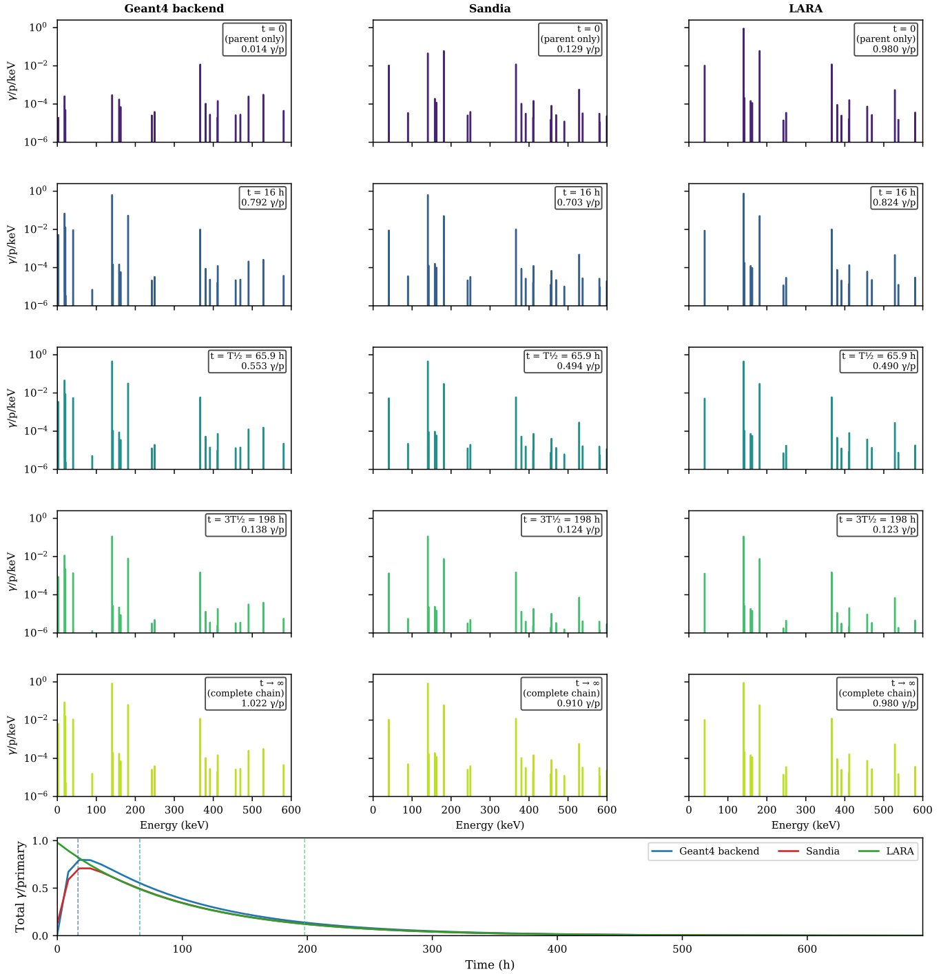
Fig. 17: ^{99}\text{Mo}/^{99m}\text{Tc} time-dependent spectra. Columns: Geant4 backend, Sandia, LARA. Rows: t = 0 (parent only – no daughter accumulated), 16 h ( \approx T_{1/4} ), T_{1/2} , 3T_{1/2} , complete chain ( t \rightarrow \infty , all descendants followed to stability). Bottom strip: total \gamma /primary vs time (h). The 140.5 keV ^{99m}\text{Tc} line ingrows non-trivially: ^{99m}\text{Tc} is fed only by the 87.7% branch of ^{99}\text{Mo} (the remaining 12.3% bypasses the isomer), so the ingrowth rate is the difference of two exponentials with T_{1/2} values 65.9 h and 6.0 h. The LARA backend starts at \approx 1.15 \gamma /primary at t = 0 and remains flat across all snapshots because the LARA data file for ^{99}\text{Mo} bundles all cascade emissions—including the 140.5 keV ^{99m}\text{Tc} line—directly into ^{99}\text{Mo} 's emission list; no separate ^{99m}\text{Tc} chain member is constructed from LARA data. The Geant4 and Sandia backends correctly separate parent and daughter emissions and show Tc-99m ingrowth from zero.
