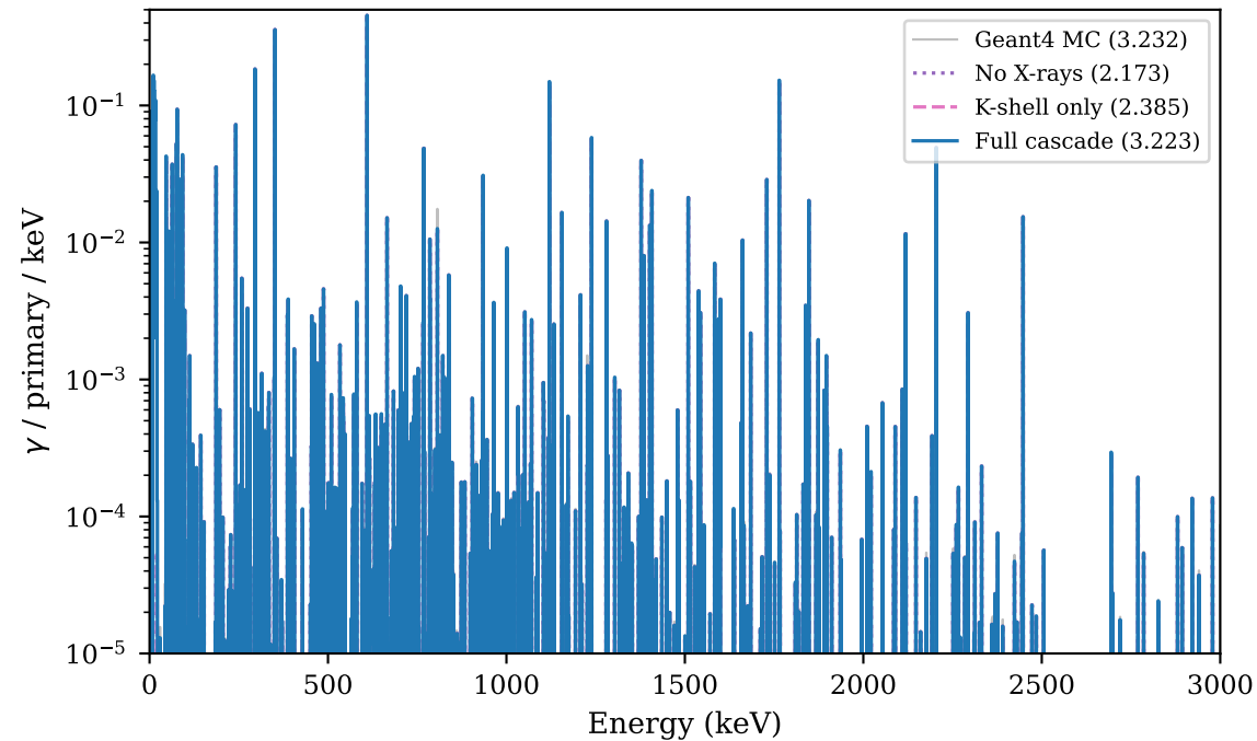
^{238}\text{U} SE - X-ray/Auger settings (full range)
