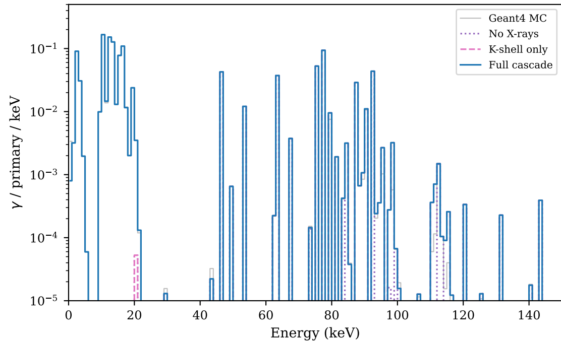
^{238}\text{U} SE - low-energy region (X-ray / Auger lines)
