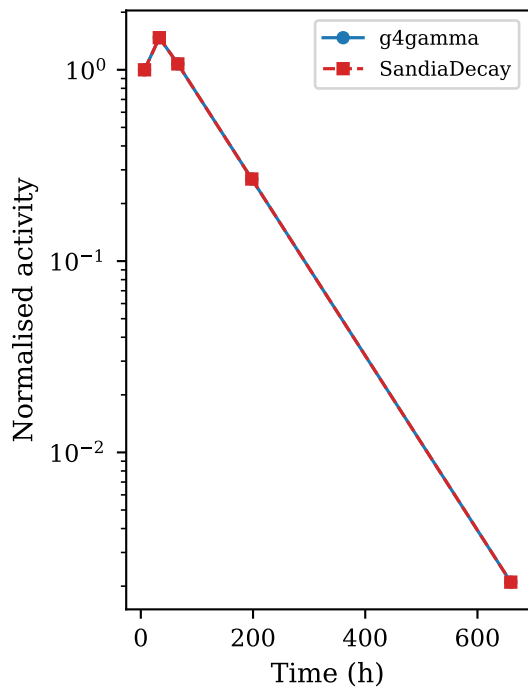
Mo99→Tc99m
