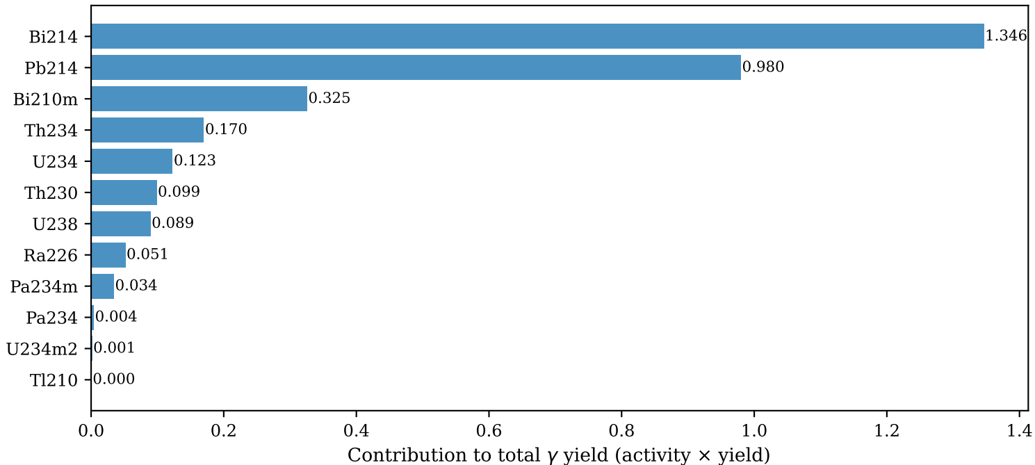
^{238}\text{U} SE - top contributing chain members (Geant4 backend)
