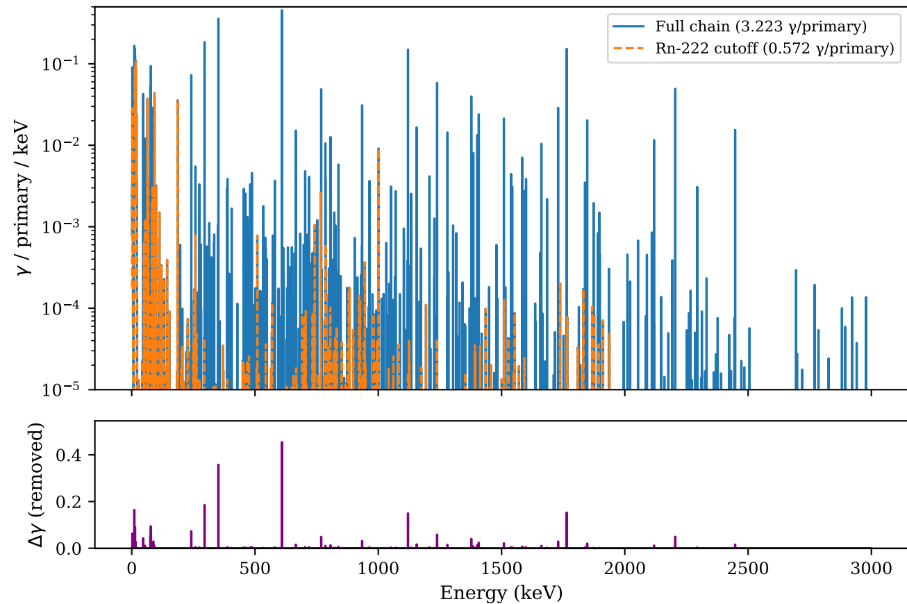
^{238}\text{U} secular equilibrium - effect of ^{222}\text{Rn} chain cutoff (radon escape)
