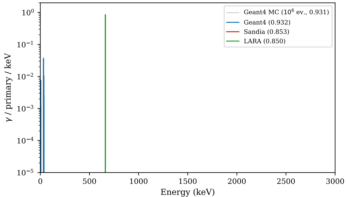
^{137}\text{Cs} secular equilibrium (legend shows \gamma /primary total)
