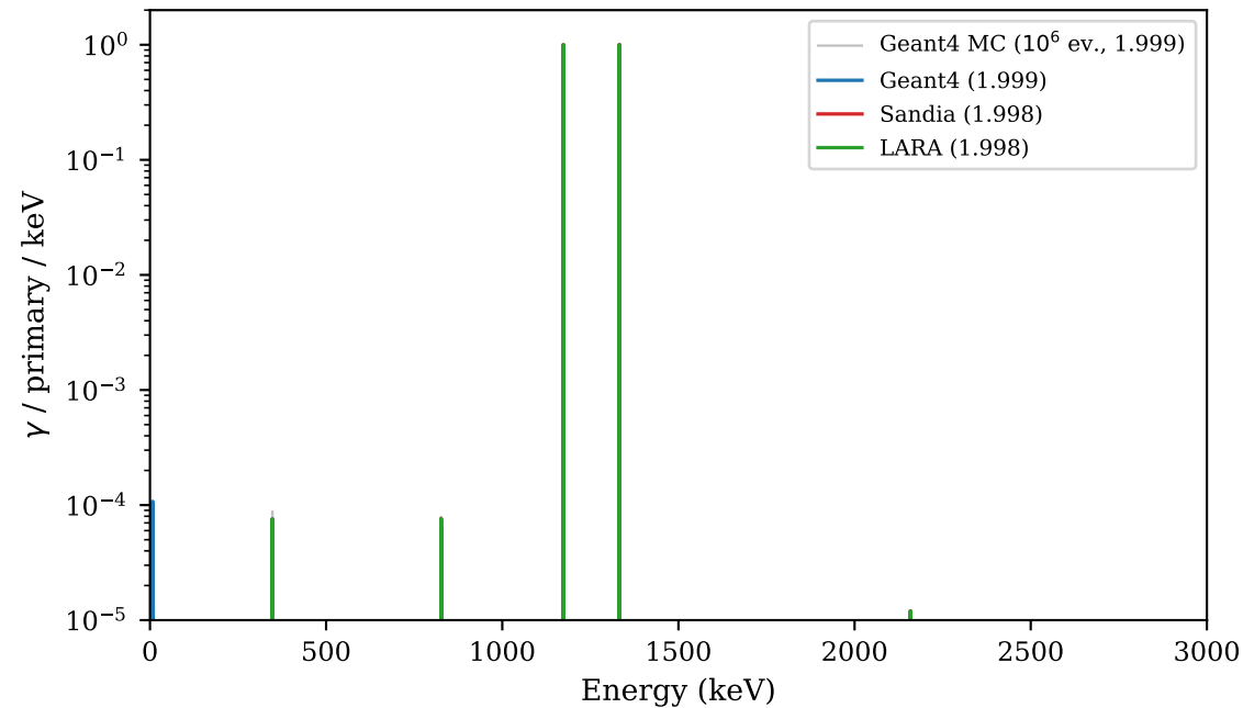
^{60}\text{Co} secular equilibrium (legend shows \gamma /primary total)
