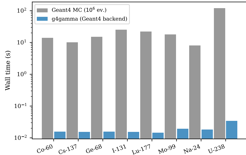
Computation time comparison
