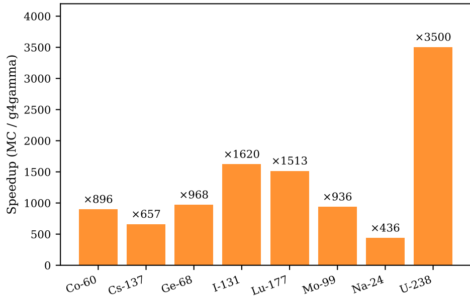
g4gamma speedup over Geant4 MC
