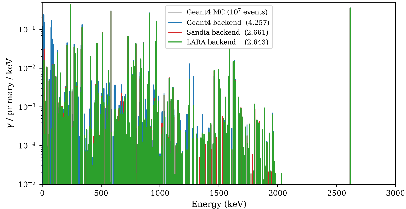
^{232}\text{Th} secular equilibrium - database comparison (legend shows \gamma /primary total)
