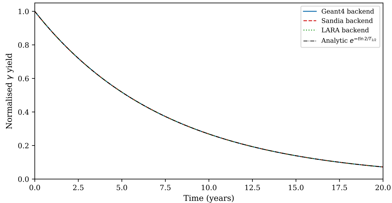
^{60}\text{Co} total \gamma yield vs time - database comparison
