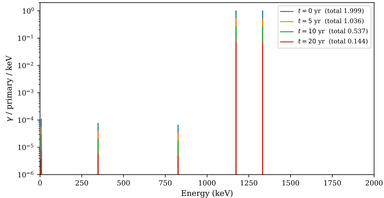
^{60}\text{Co} gamma spectrum evolution over time (Geant4 backend)
