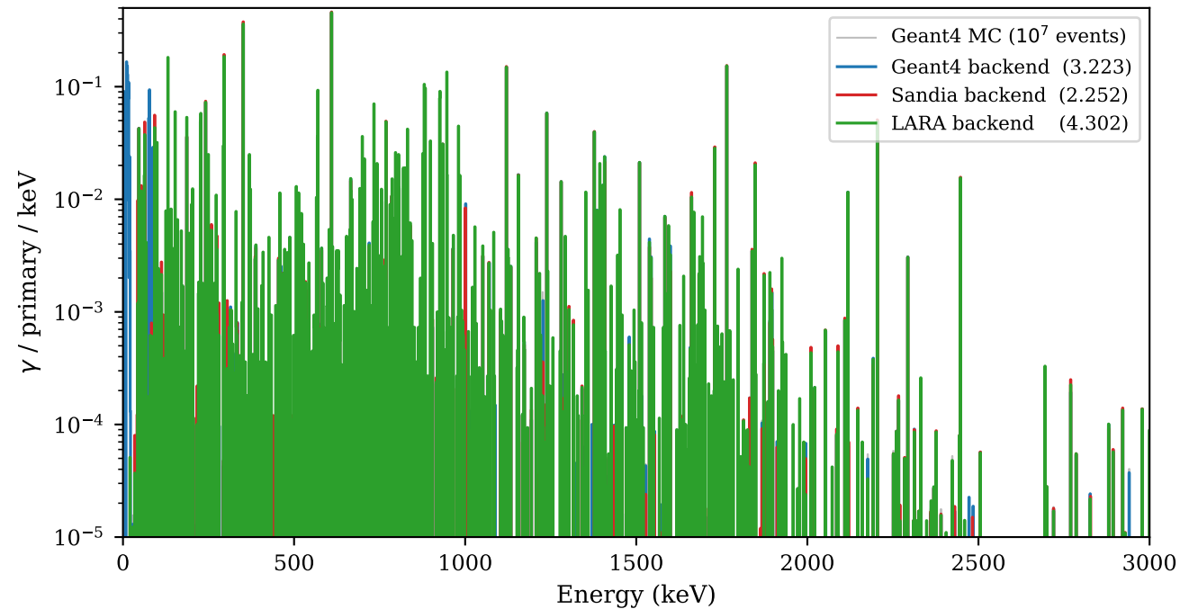
^{238}\text{U} secular equilibrium - database comparison (legend shows \gamma /primary total)
