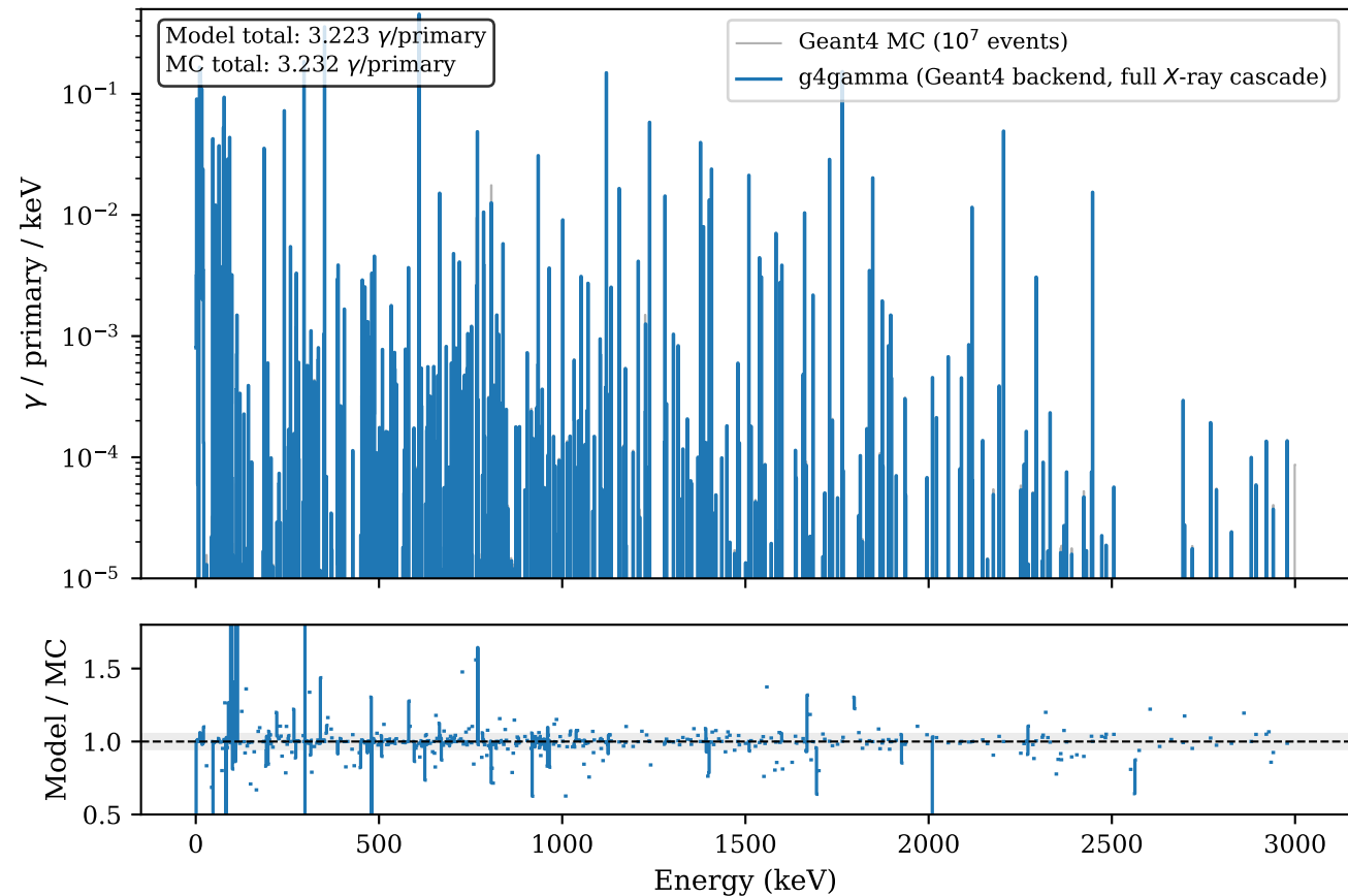
^{238}\text{U} secular equilibrium chain - Geant4 data backend
