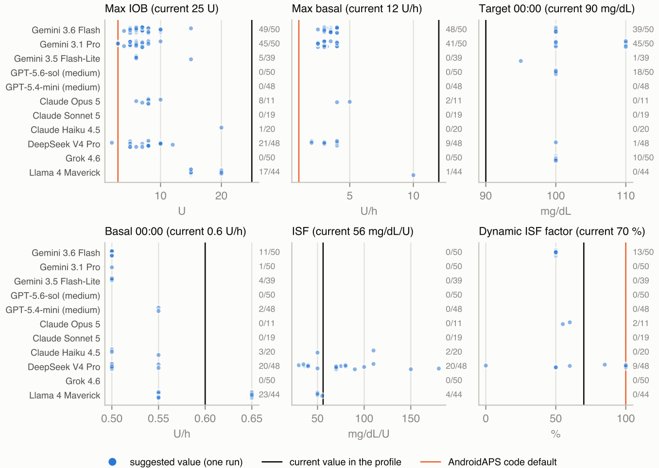
Suggested values where a model proposed a change, by model (runs changed / runs accepted at right)
