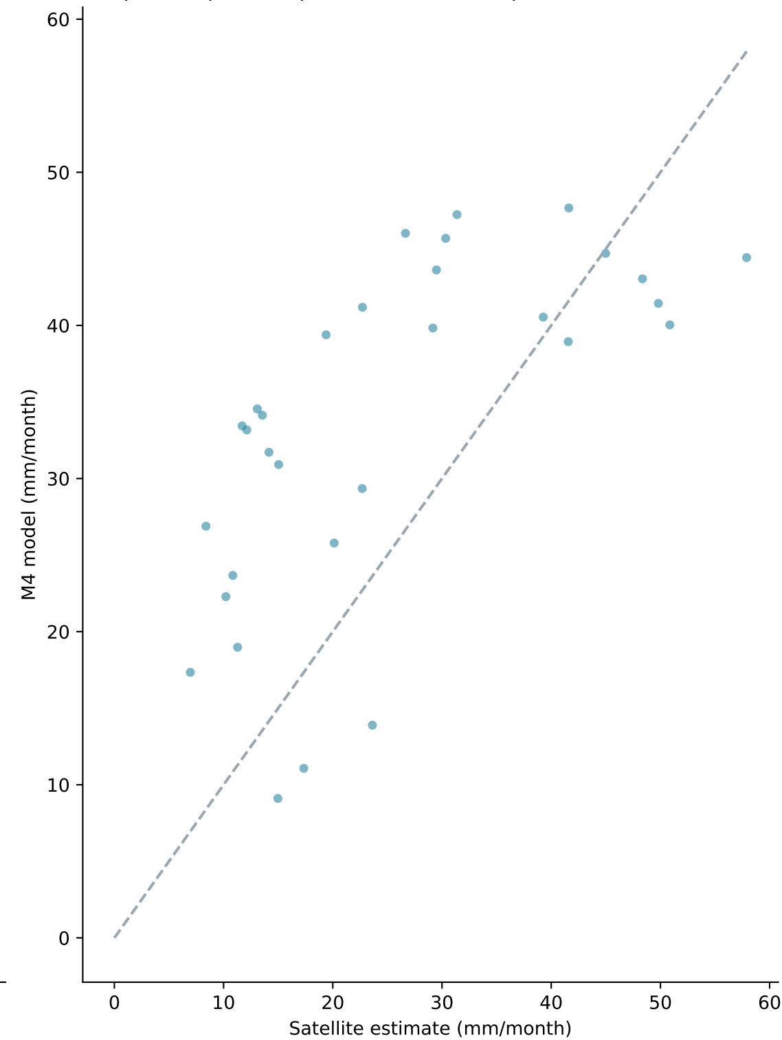
Evapotranspiration process check · 31 pairs
