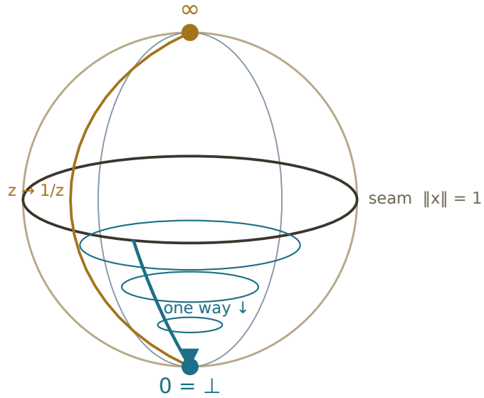
Figure 1. The p -adic Riemann sphere. The poles 0 = \perp (the floor) and \infty (the ceiling) are antipodal; the equator \|x\| = 1 is the seam. Inside \mathbb{Z}_p (the lower hemisphere) the \omega -tower falls one way to 0; the inversion z \rightarrow 1/z (rInv) swaps the poles 0 \leftrightarrow \infty — continuous on the sphere, torn at 0 in the field.
