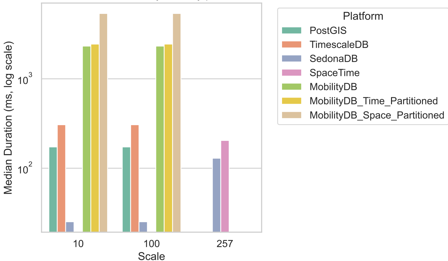
Avi.Q2 - Median Query Latency per Scale
