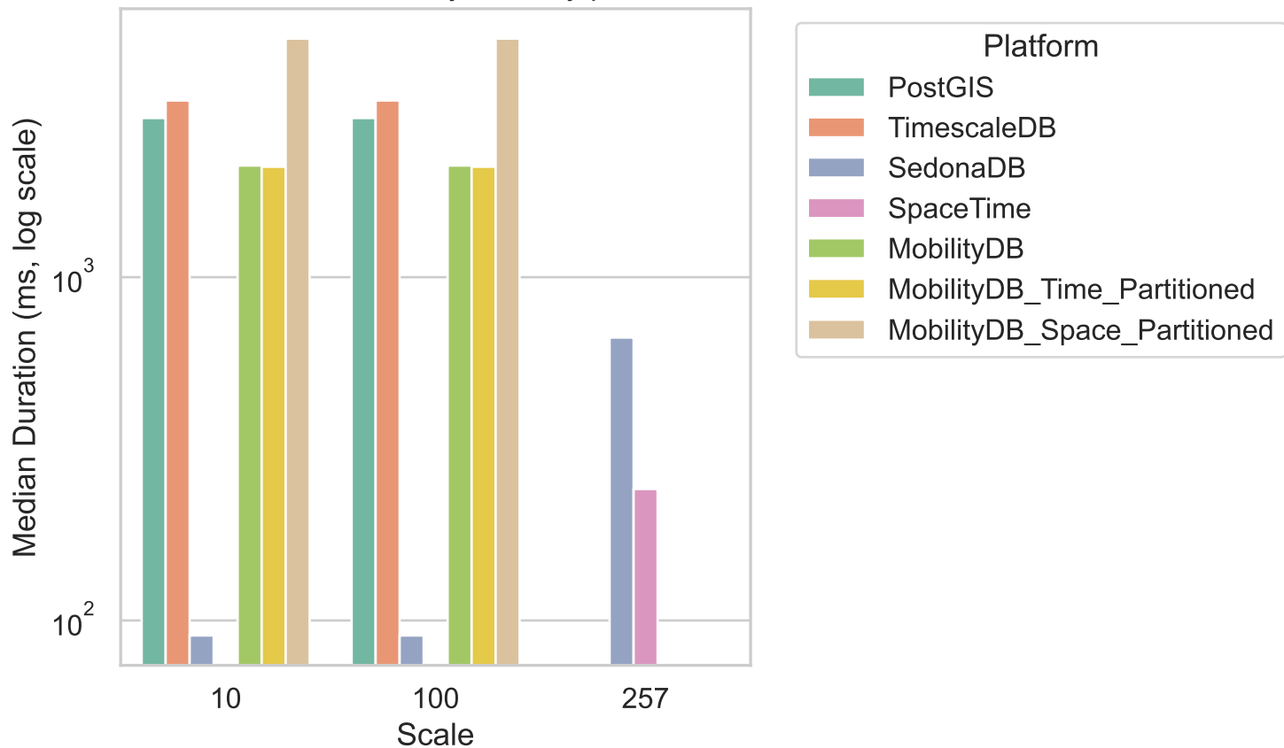
Avi.Q5 - Median Query Latency per Scale
