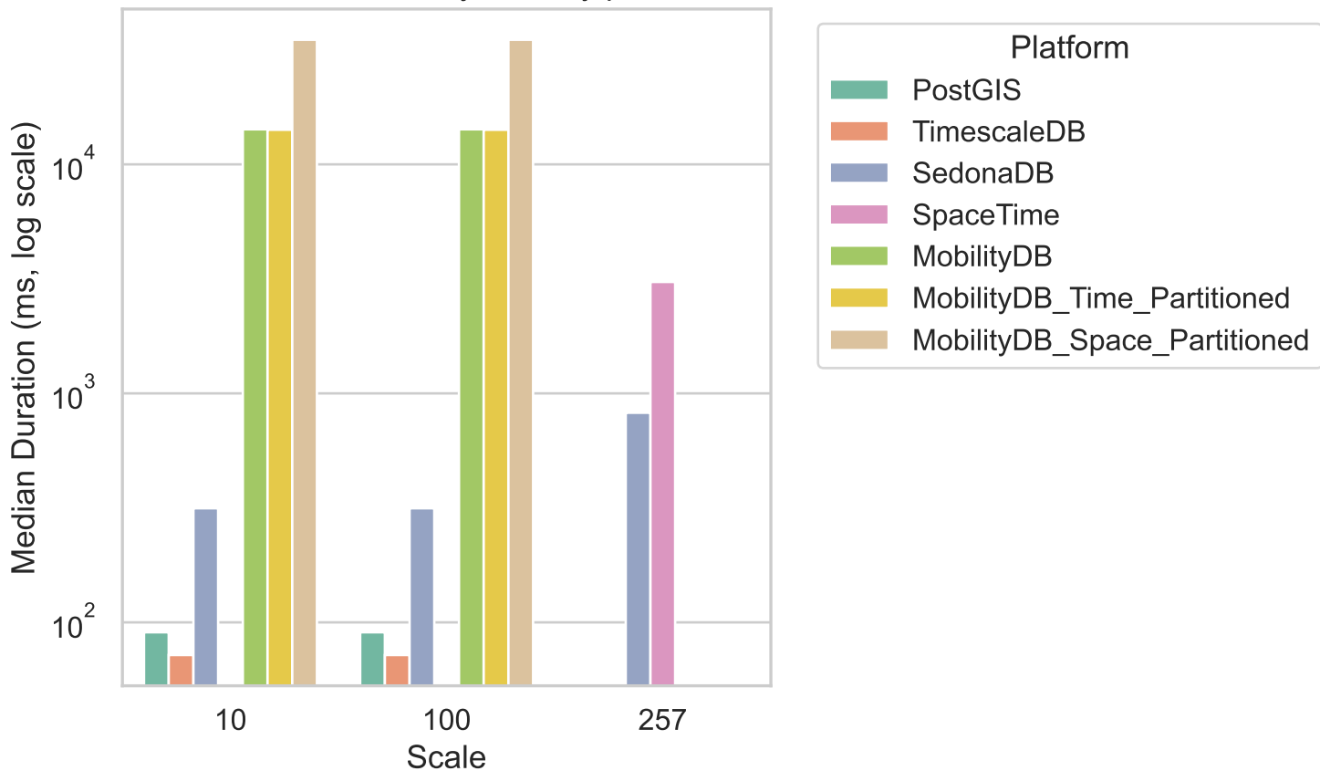
Avi.Q4 - Median Query Latency per Scale
