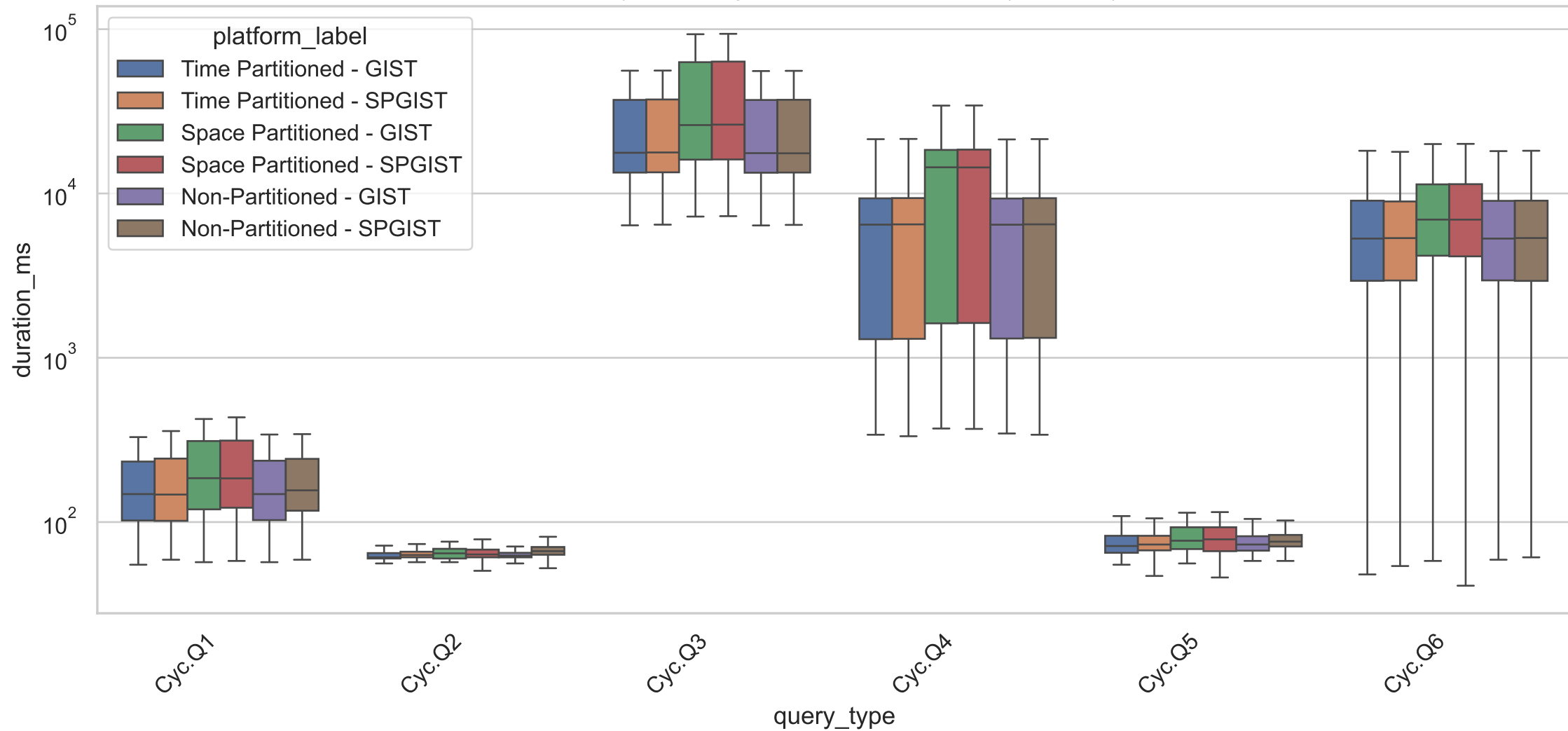
MobilityDB Config Comparison – Boxplot (ID=c0fbe)
