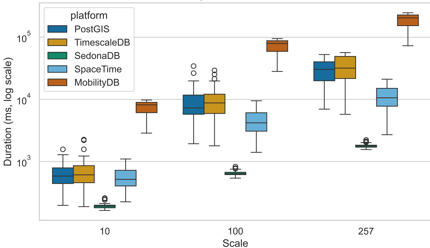
Latency Distribution – Avi.Q3
