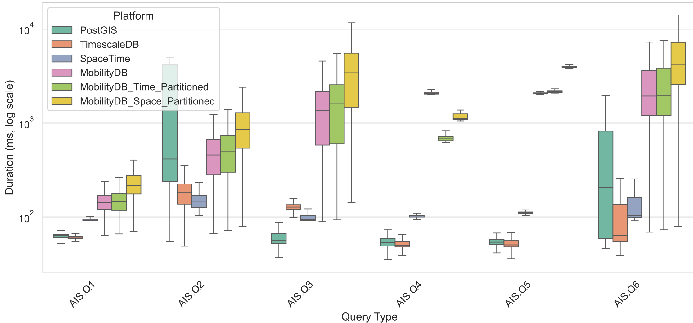
Query Performance Comparison by Platform – 96e2c
