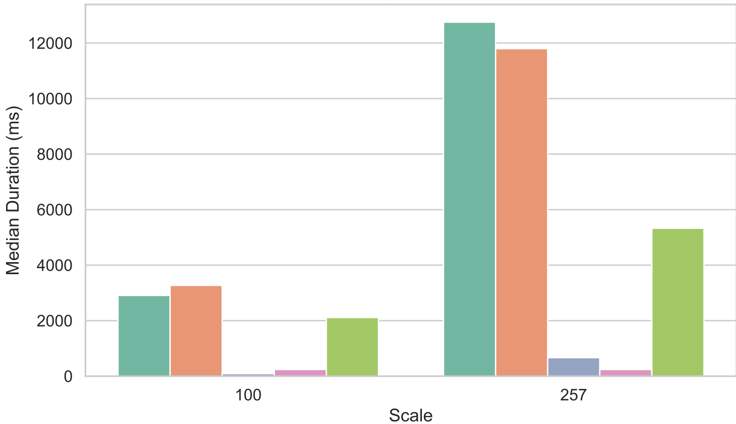
Median Query Latency -- Avi.Q5
