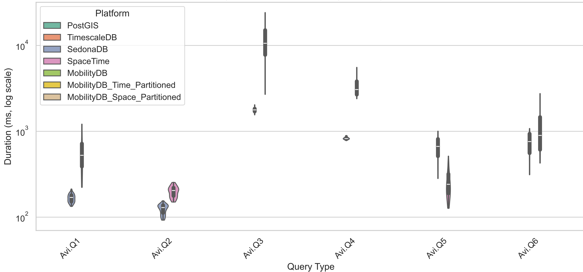
Query Performance Distribution (Violin Plot) – 11111
