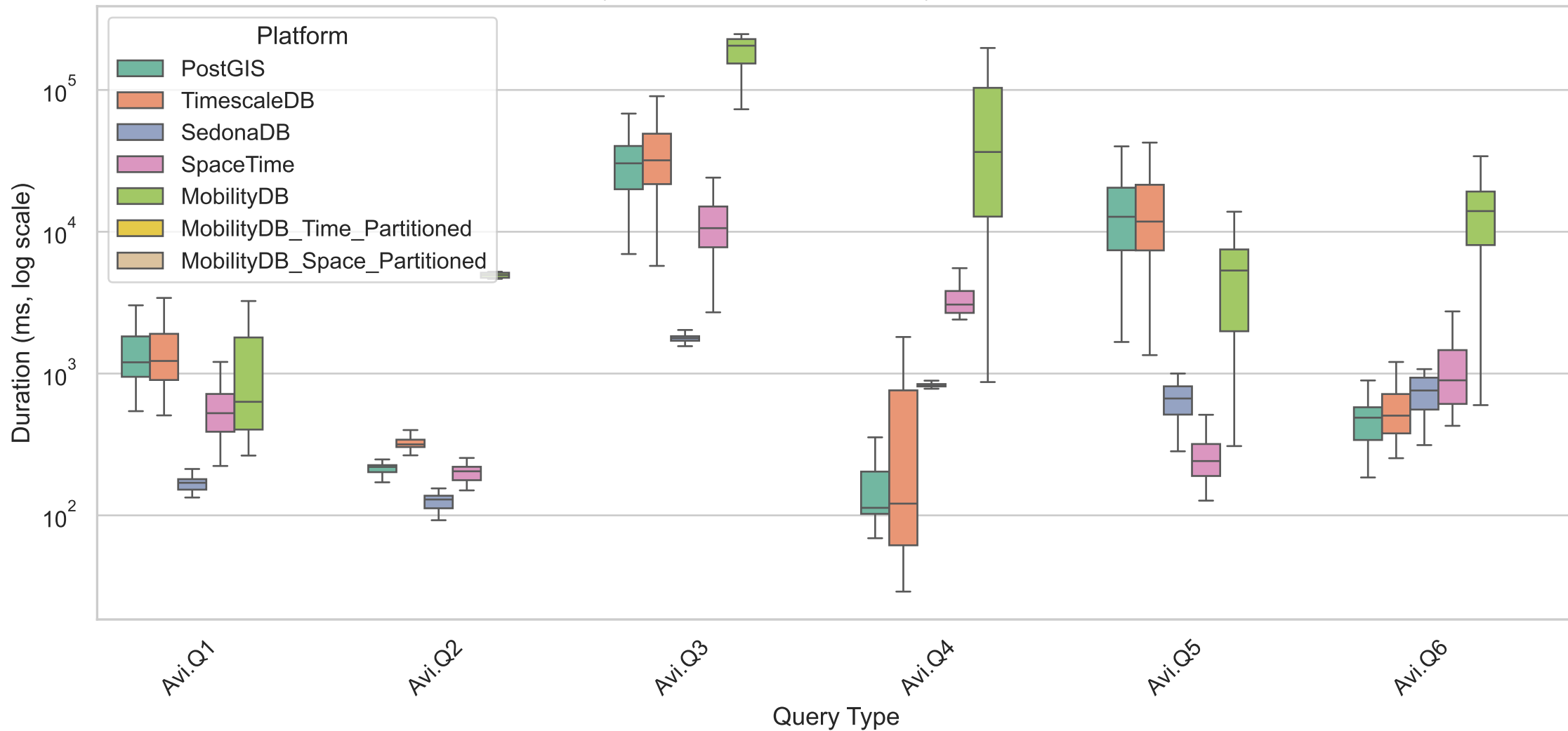
Query Performance Comparison by Platform – 11111
