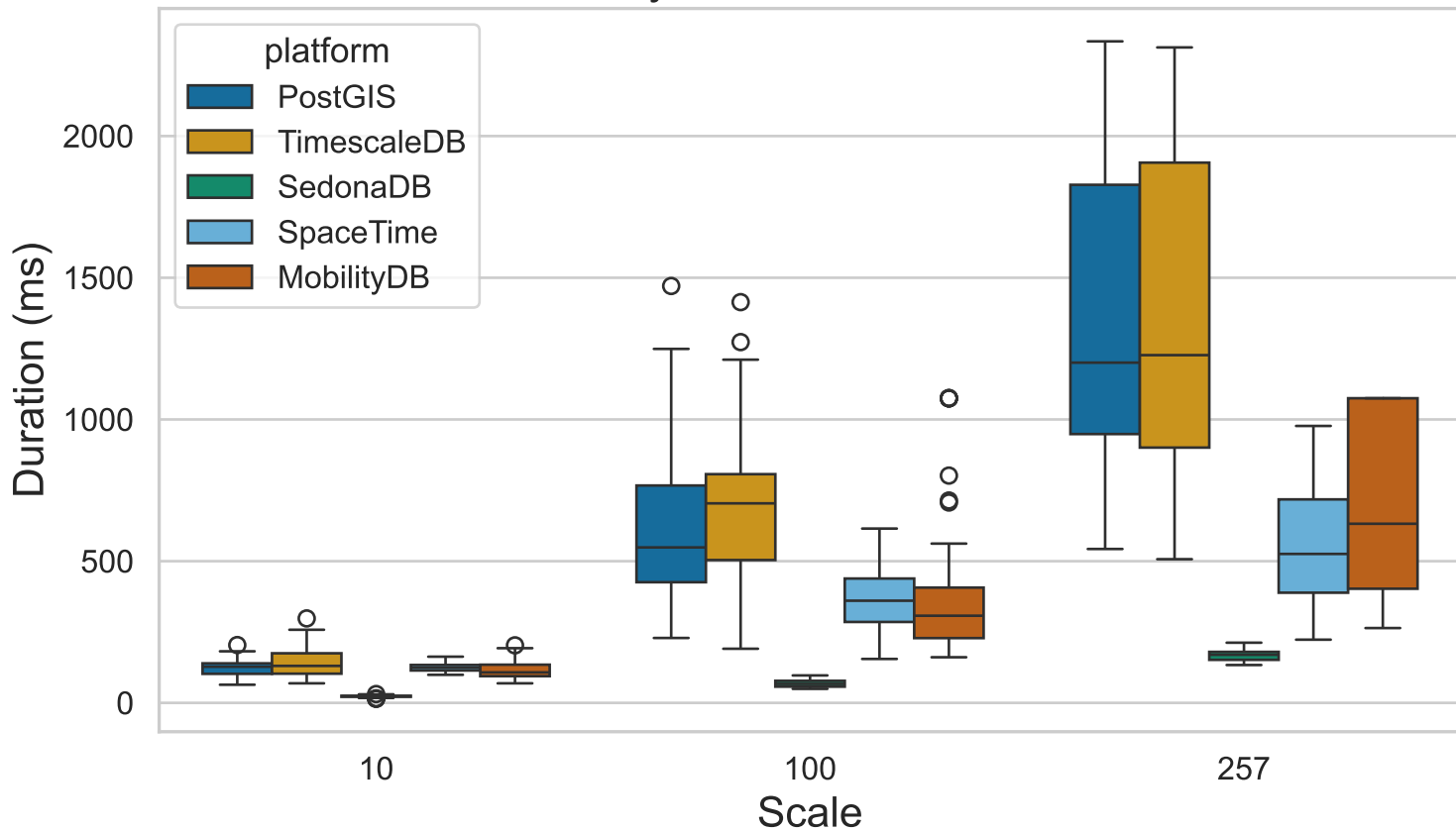
Latency Distribution – Avi.Q1
