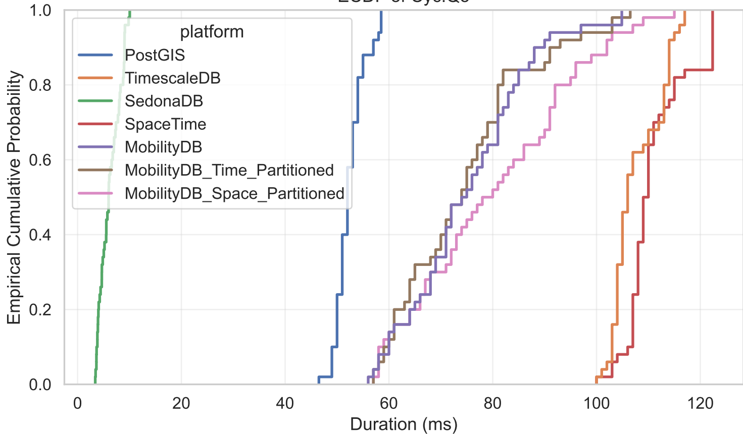
ECDF of Cyc.Q5
