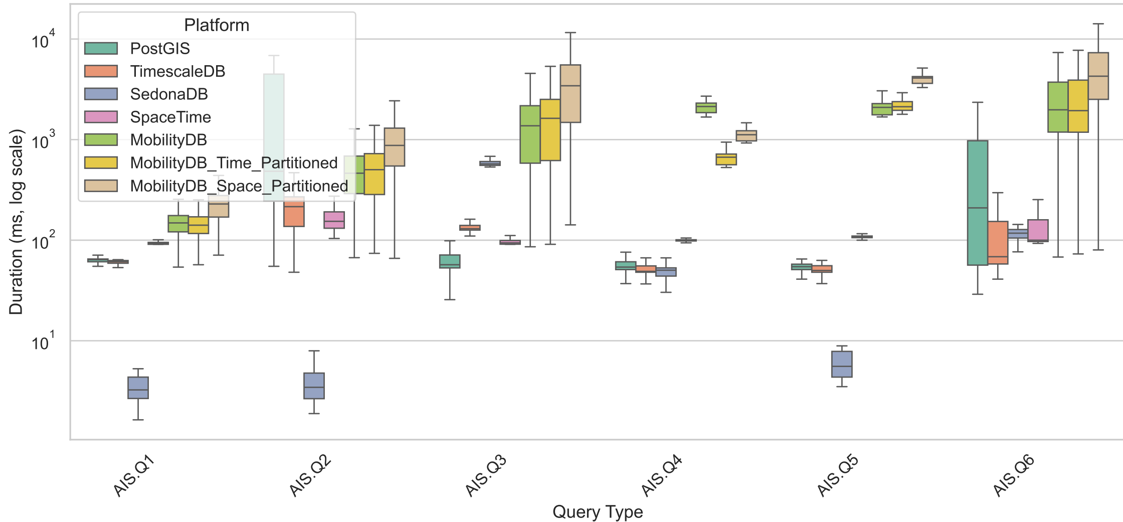
Query Performance Comparison by Platform – 9430d
