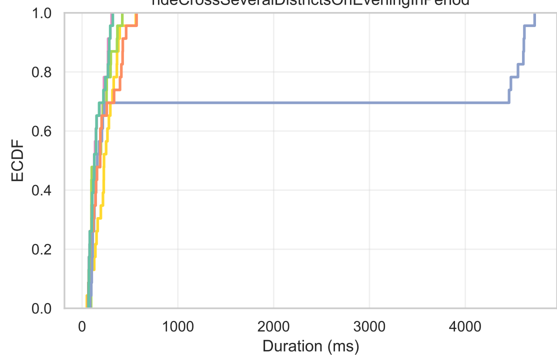
rideCrossSeveralDistrictsOnEveningInPeriod
