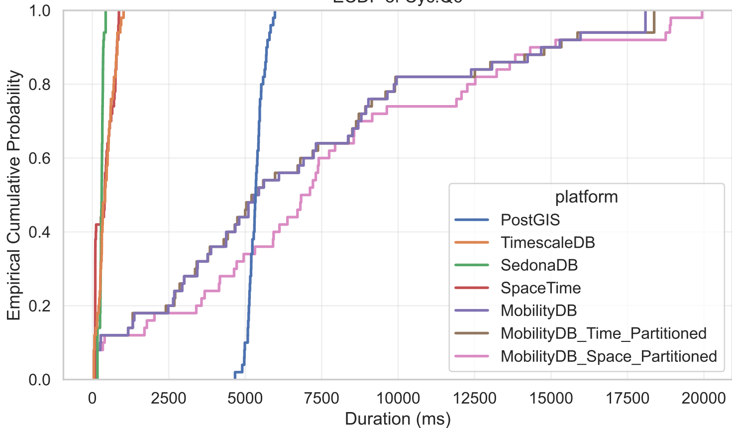
ECDF of Cyc.Q6
