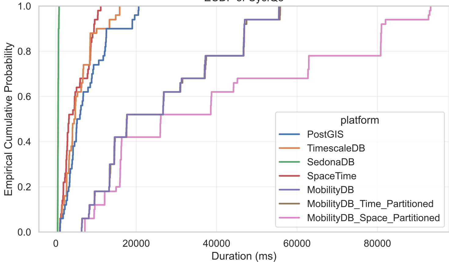
ECDF of Cyc.Q3
