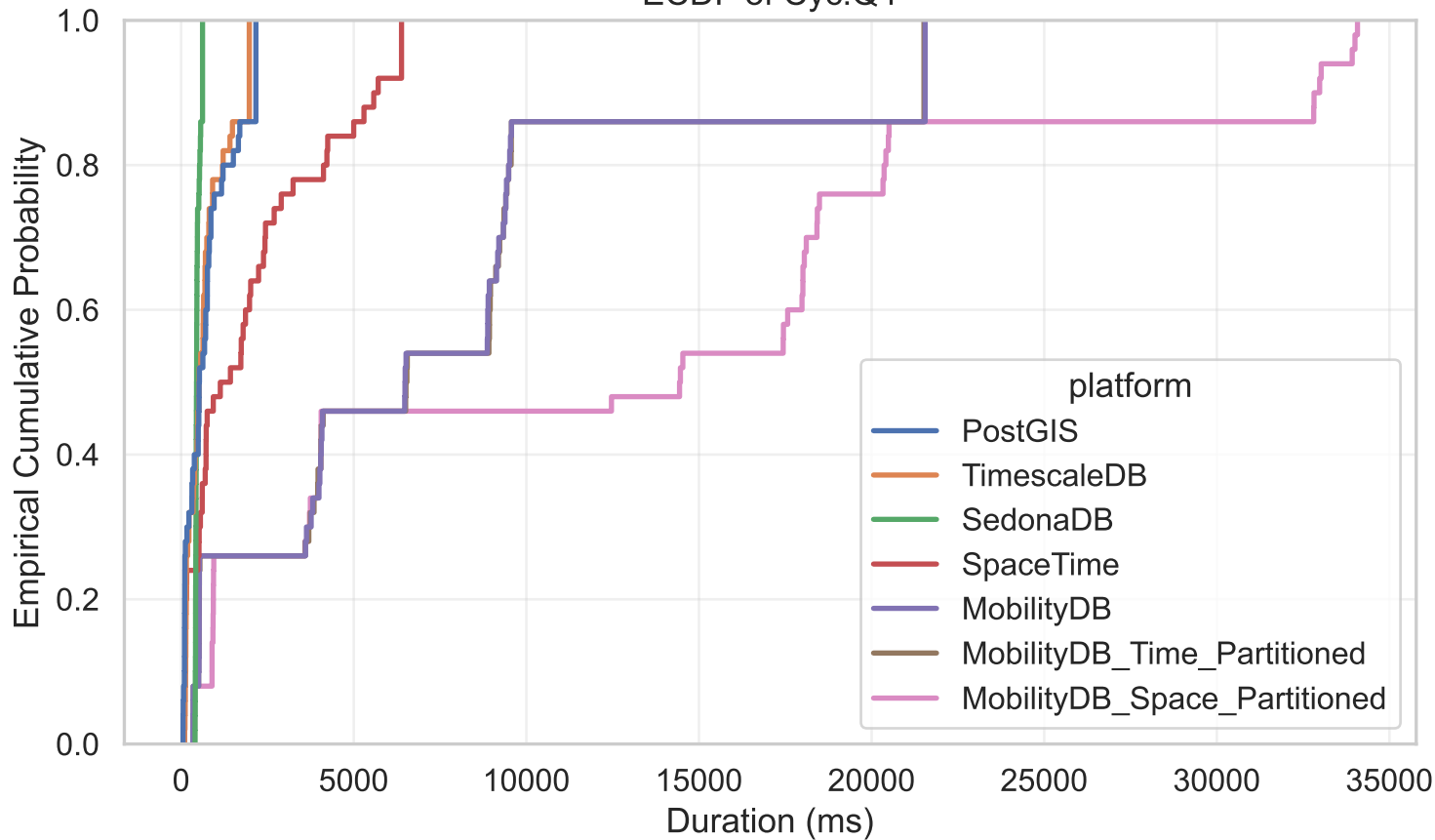
ECDF of Cyc.Q4
