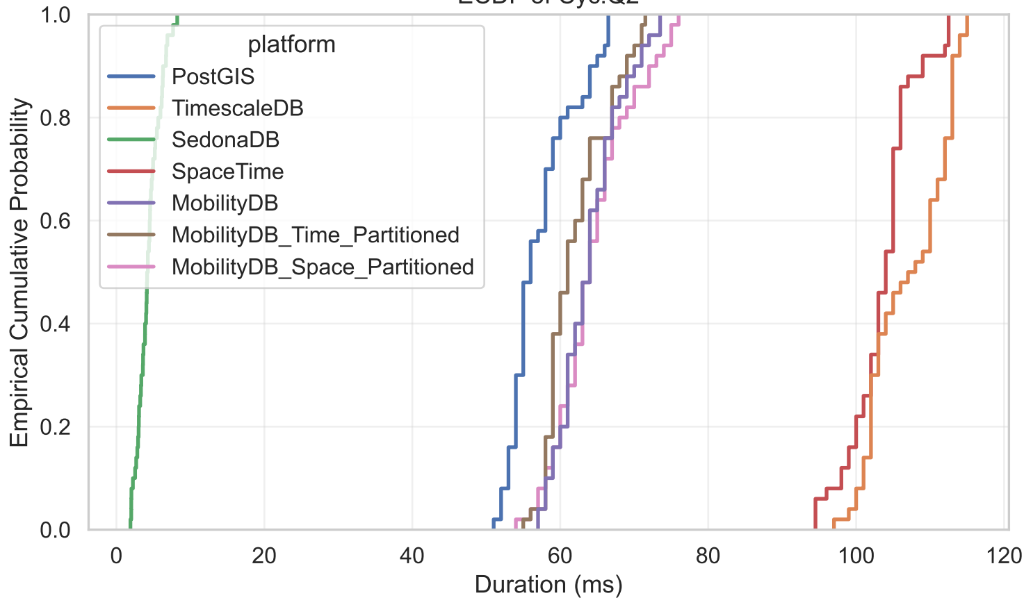
ECDF of Cyc.Q2
