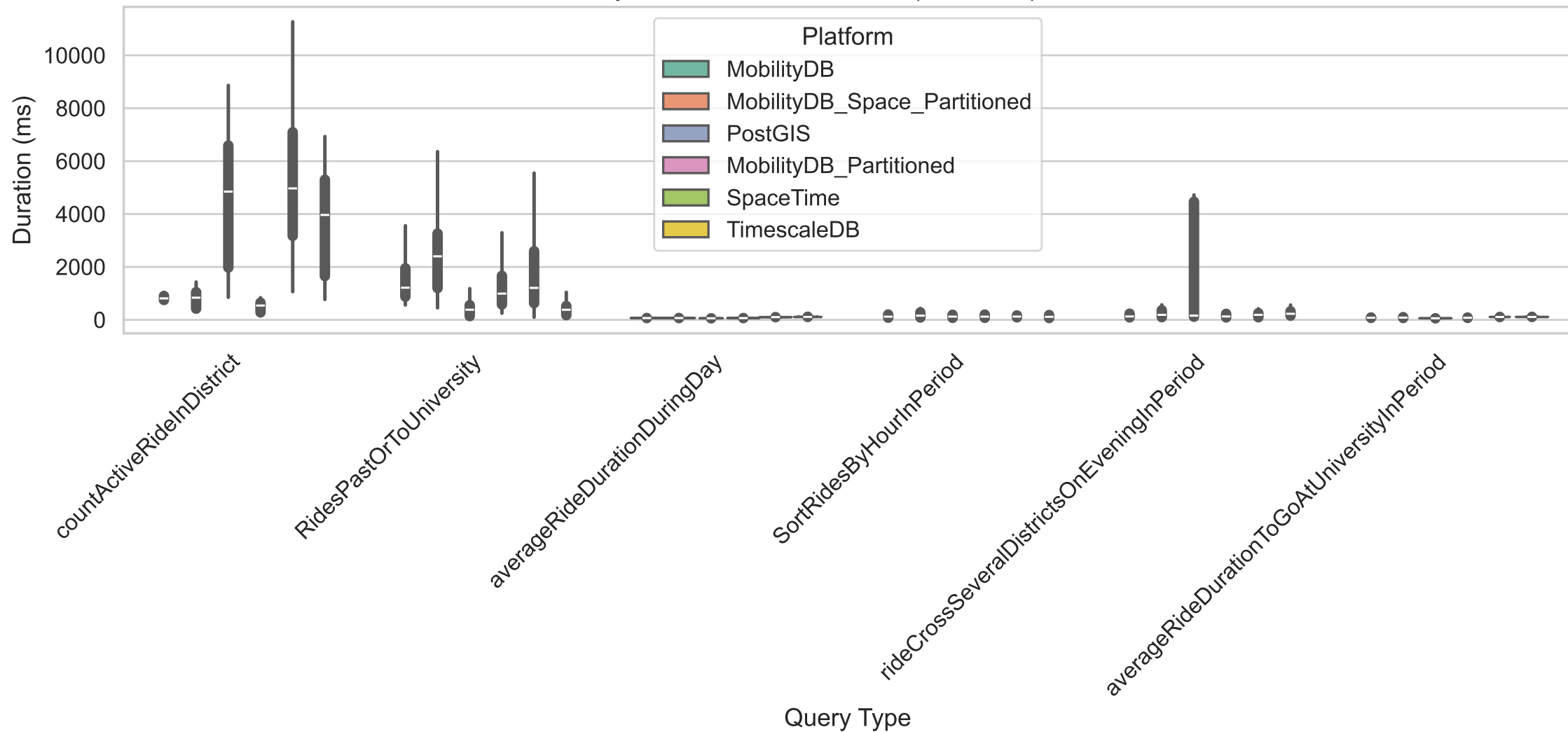
Query Performance Distribution (Violin Plot) – 80b8e
