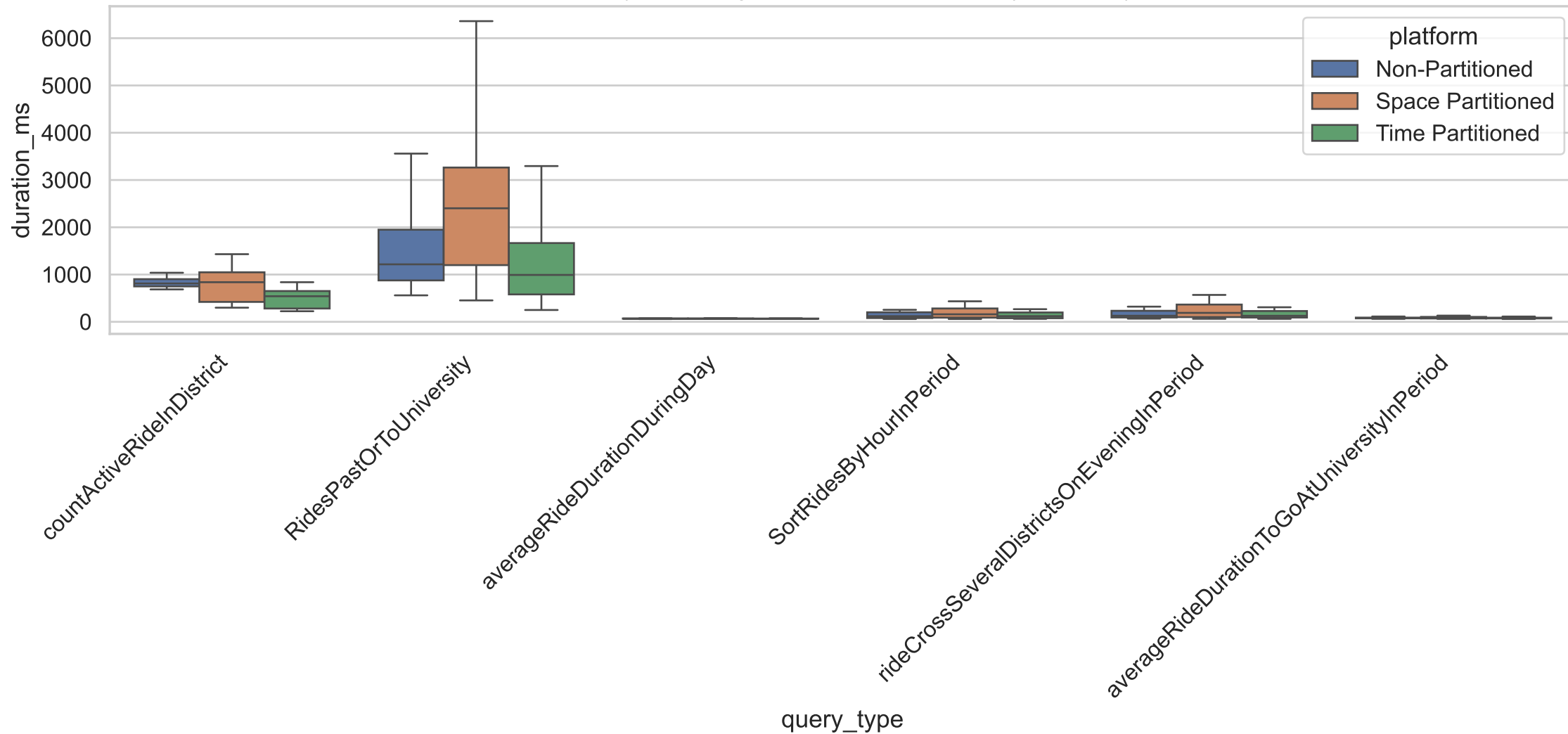
MobilityDB Config Comparison – Boxplot (ID=80b8e)
