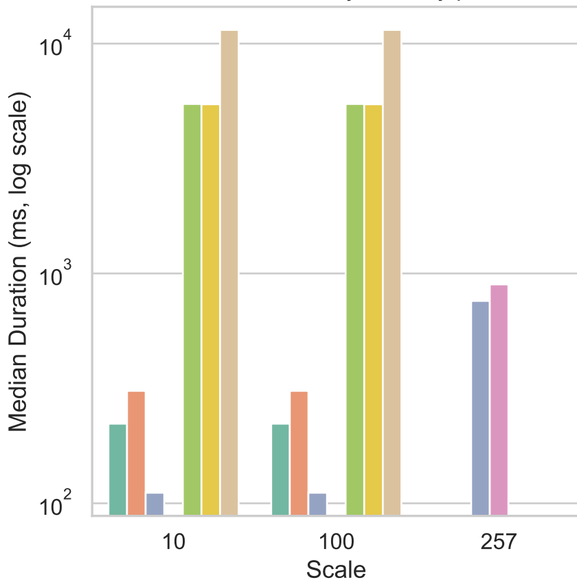
Avi.Q6 - Median Query Latency per Scale
