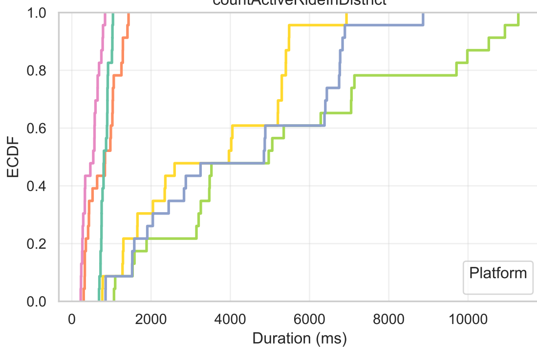
countActiveRideInDistrict
