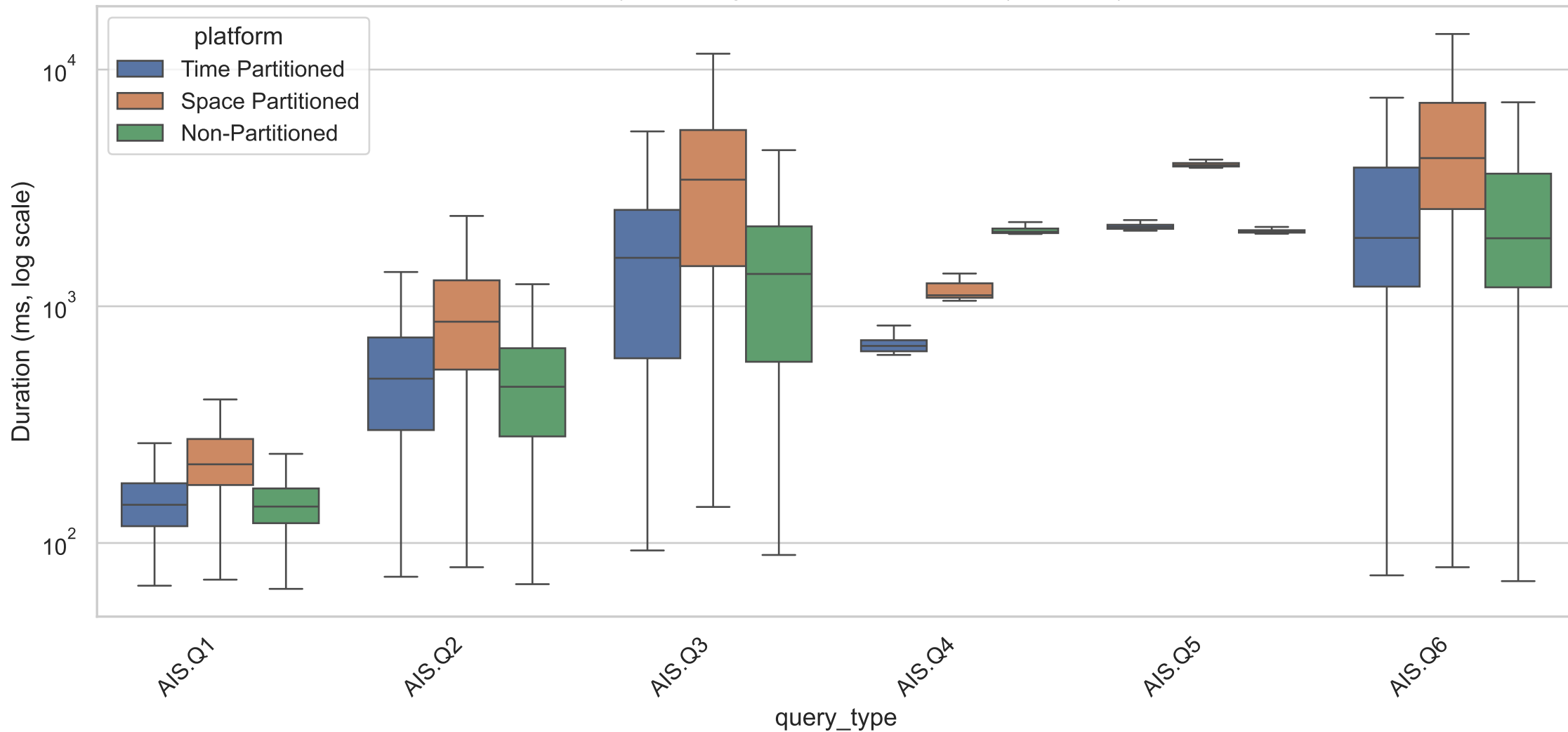
MobilityDB Config Comparison – Boxplot (ID=96e2c)
