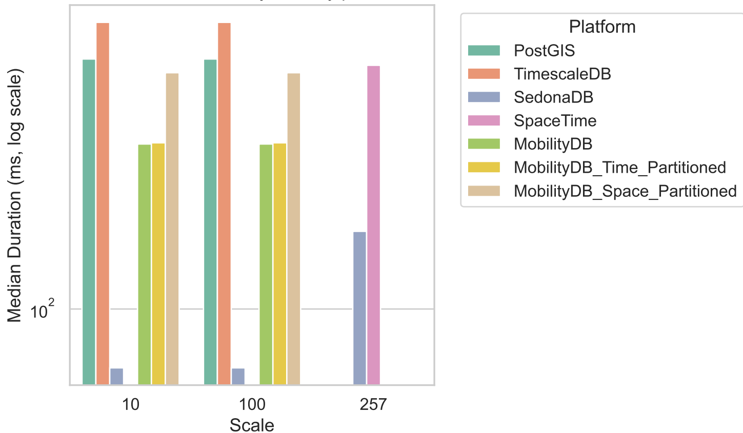
Avi.Q1 - Median Query Latency per Scale
