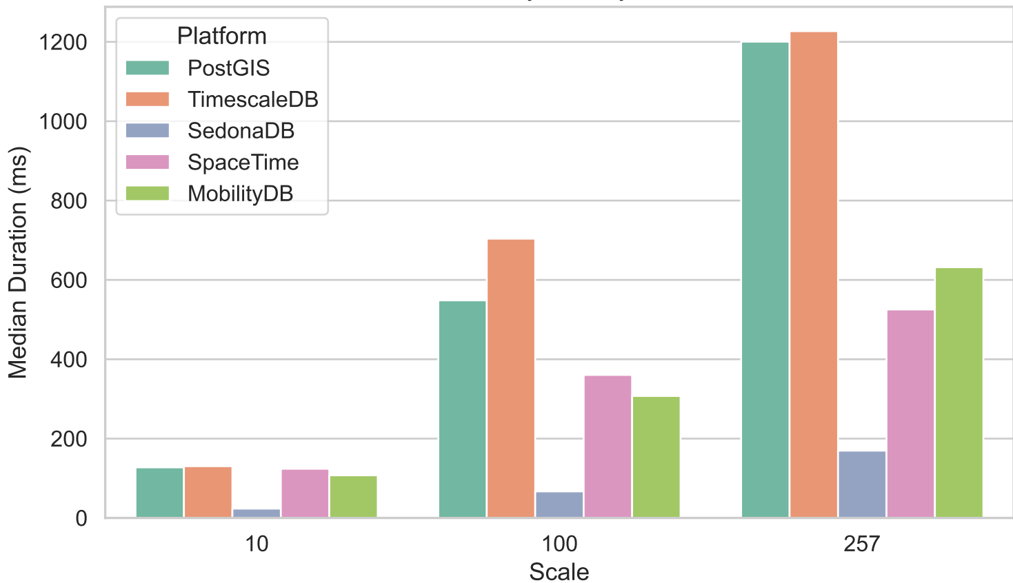
Median Query Latency -- Avi.Q1
