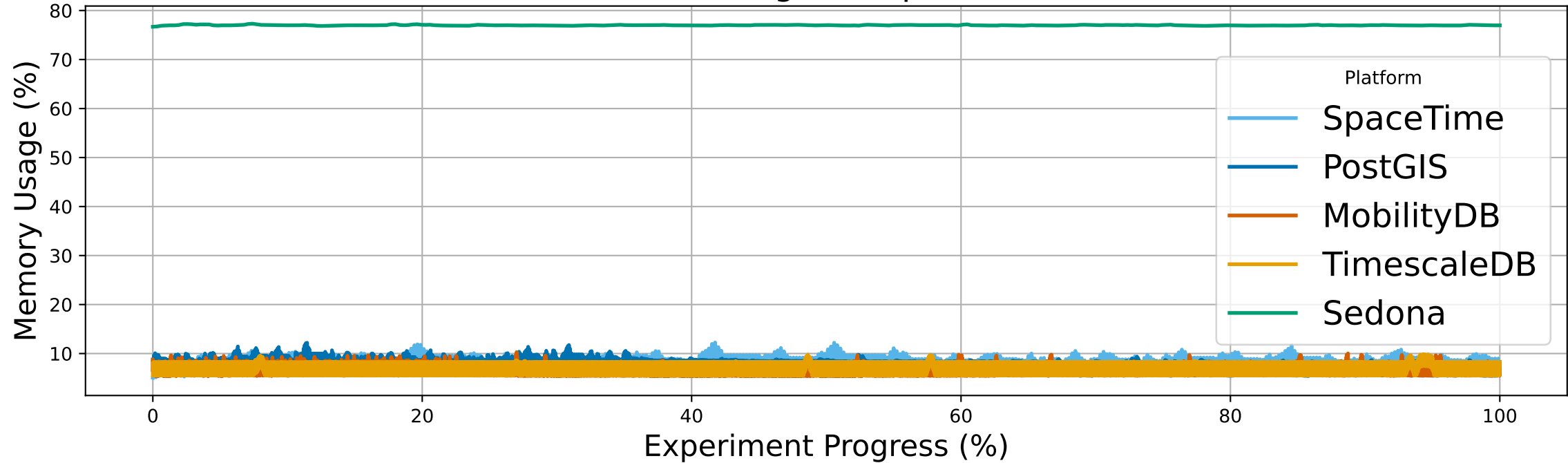
RAM Usage Comparison
