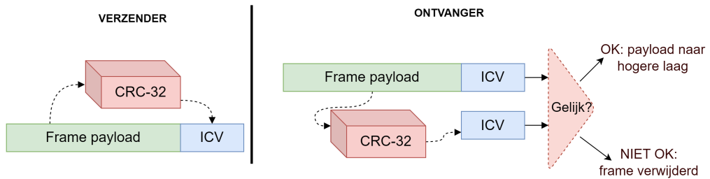
Figuur 5.10: Integrity check.
