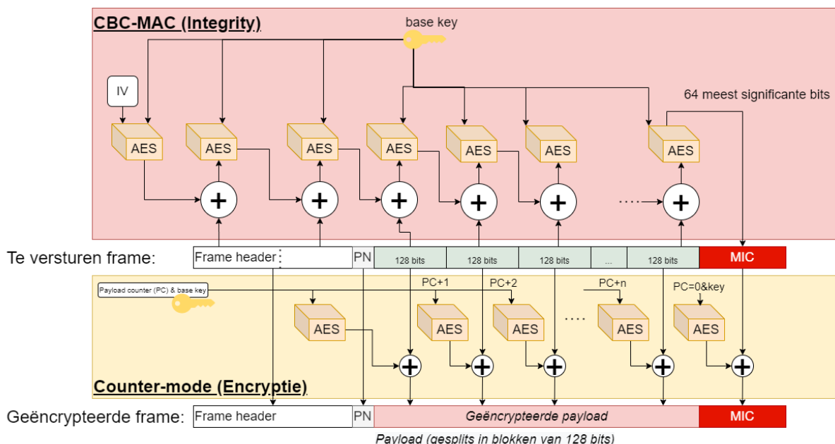
Figuur 0.23: CCMP: confidentiality en integrity in 1
