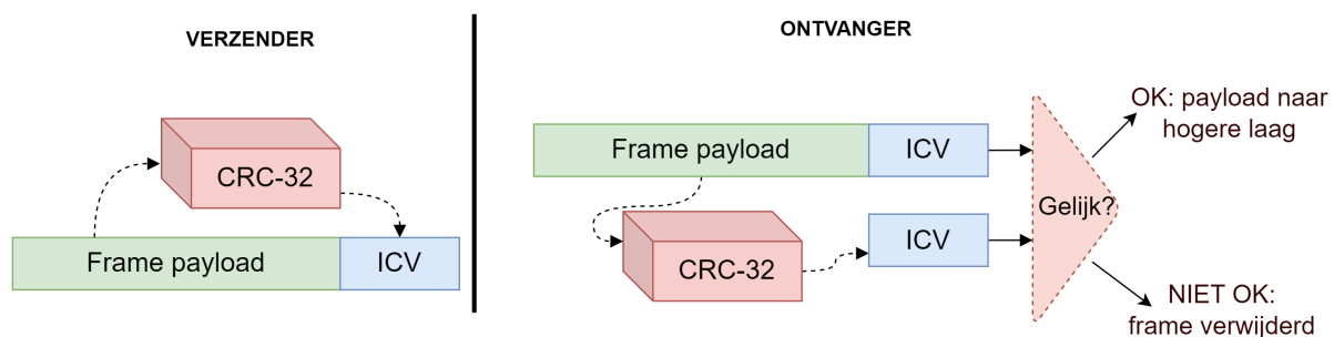
Figuur 5.9: Integrity check.
