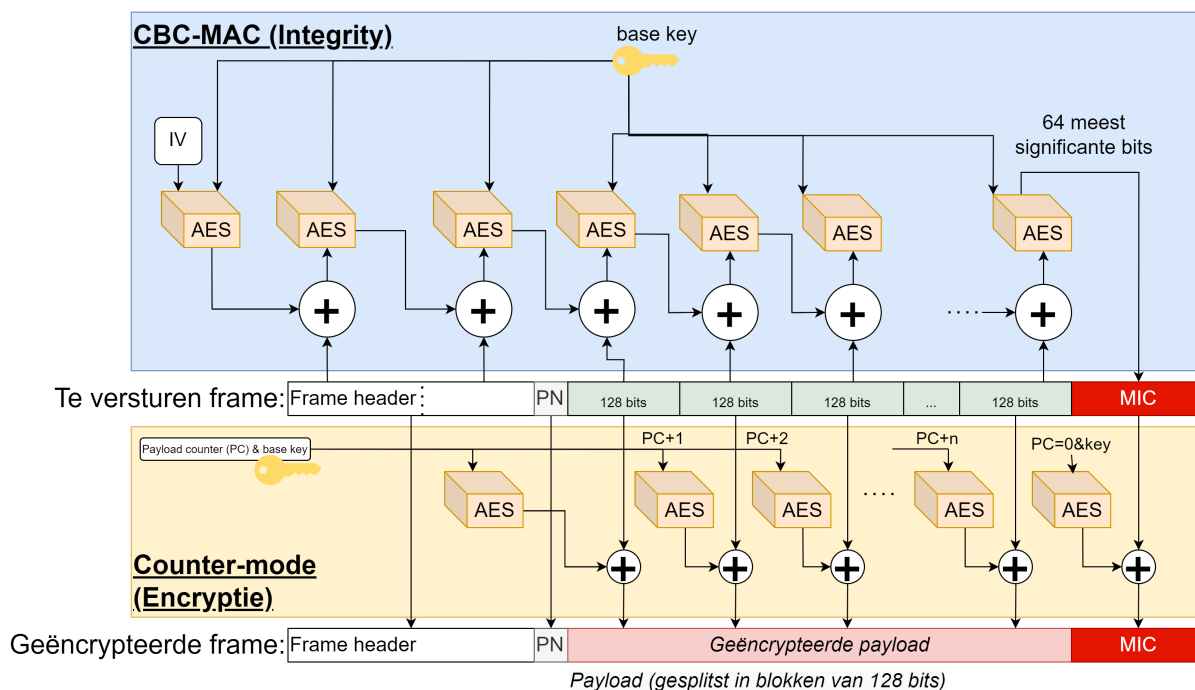
Figuur 5.23: CCMP: confidentiality en integrity in 1
