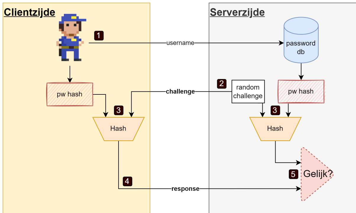
Figuur 6.7: CRAM flow.
