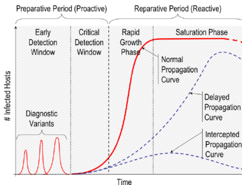
Figuur 3.14: Worm propagation model. Bron: Network Eye: End-to-End Computer Security Visualization - Scientific Figure on ResearchGate.
