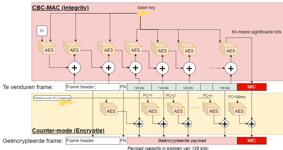
Figuur 5.23: CCMP: confidentiality en integrity in 1
