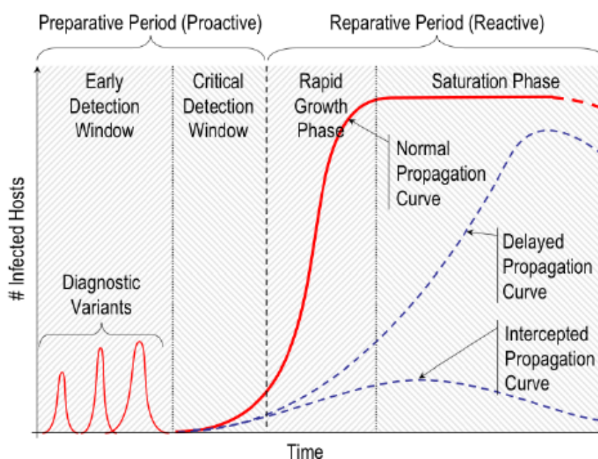
Figuur 3.13: Worm propagation model. Bron: Network Eye: End-to-End Computer Security Visualization - Scientific Figure on ResearchGate.
