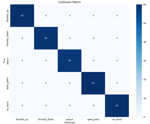
Figure 7: Confusion matrix for flip+rotate model.
