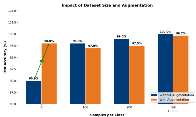
Figure 8: Impact of dataset size on accuracy. Augmentation provides an 8% boost with only 50 samples per class.
