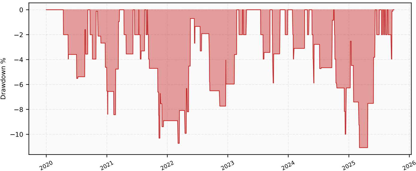
Drawdown (%)
