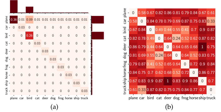
Fig. 9: (a) OT plan between two probability vectors over classes in CIFAR10 [68]. (b) Pairwise distances between Word2Vec [69] embeddings of class labels. The Wasserstein loss proposed by [70] corresponds to the Frobenius inner product between those two matrices.
