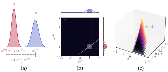
Fig. 1: Illustration of (a) Monge formulation, (b) Kantorovich formulation and (c) Benamou-Brenier formulation. While (a) focuses on transportation maps T , (b) relies on transport plans \gamma and (c) revolves around interpolations \rho(t, x) .
