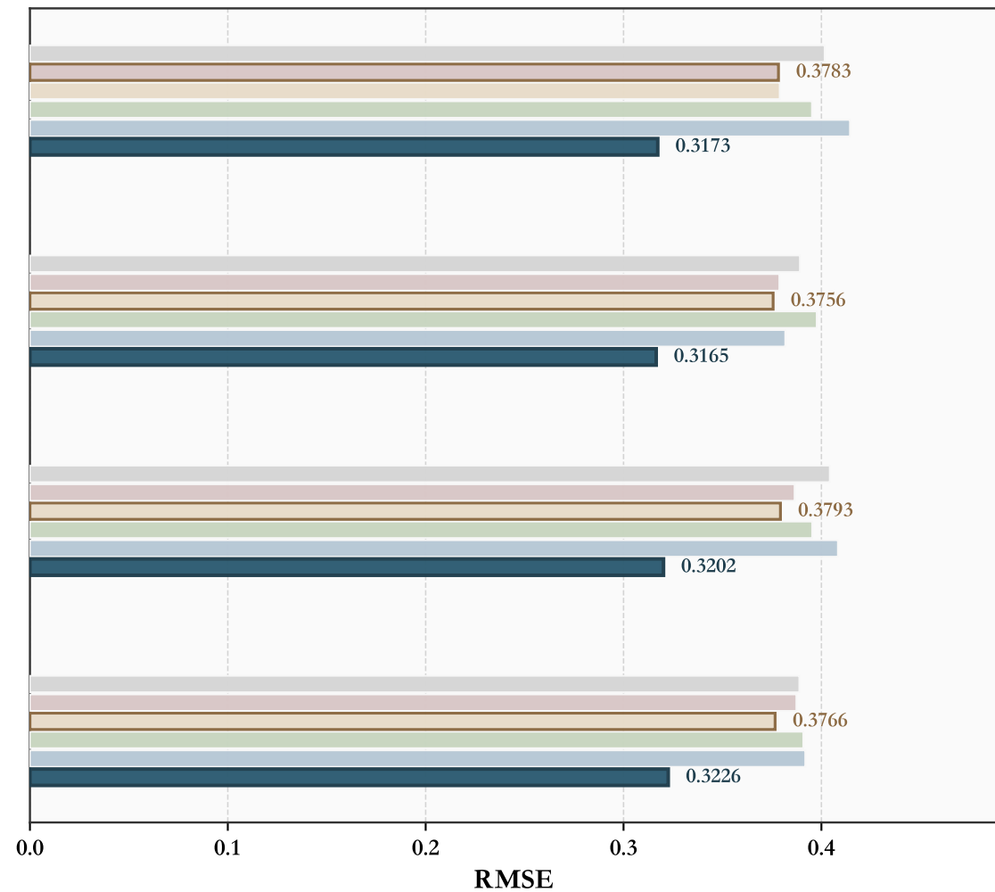
(b) RMSE
