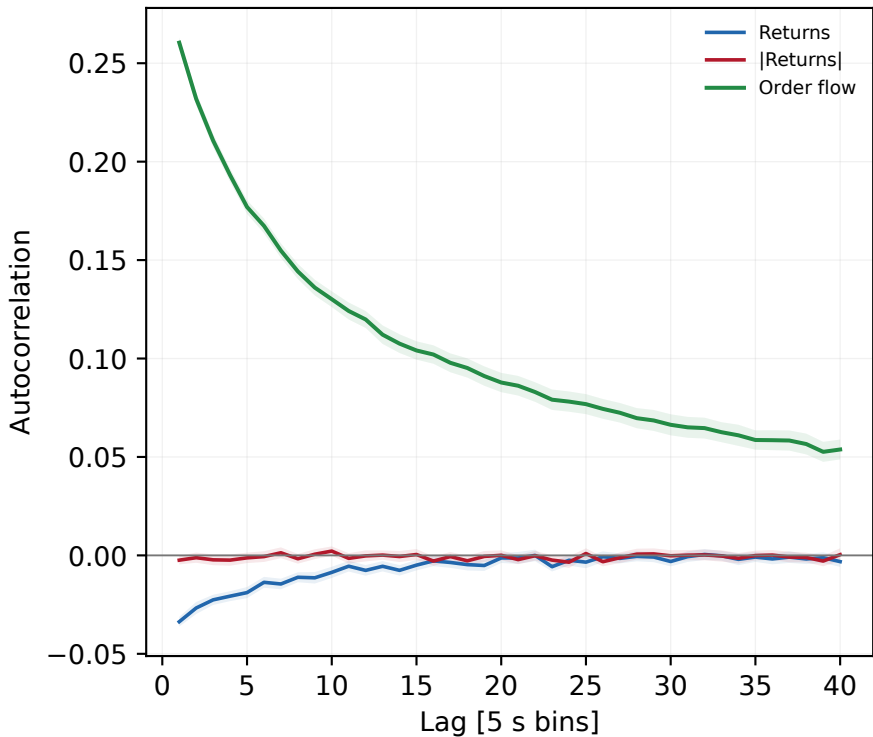
(c) Operational: acf
