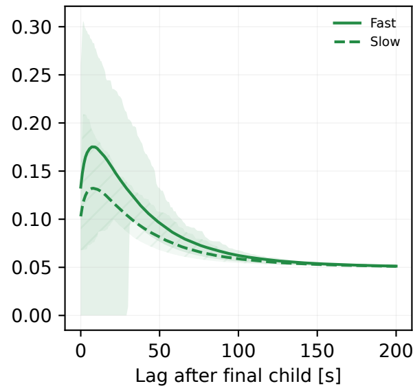
Tempered ML
