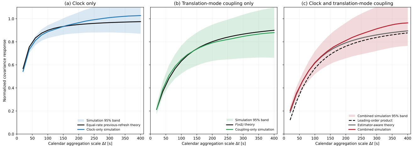
Figure 7: Final estimator-aware Epps integration. The three square panels share one linear 0–400 second and 0–1.1 normalized-covariance scale. Panel (a) shows the clock-only comparison, panel (b) shows the translation-mode coupling-only comparison, and panel (c) compares the combined no-refit holdout with the paper’s leading-order product and the exact finite-grid, finite-step conditional moment on the same realised clocks. The estimator-aware combined RMSE is 0.039719, standardized RMSE is 0.455132, and pointwise normal-band coverage is complete. No parameter, normalization or time map is refitted.
