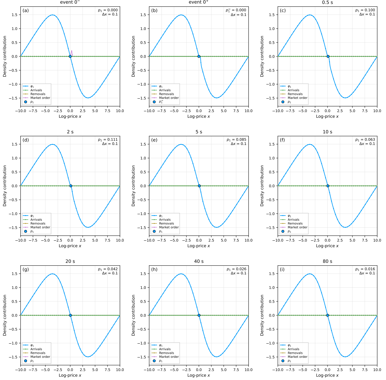
Figure 12: Fixed-time order-book shock recovery. Nine snapshots follow a buy market order in book 1 from the pre-event state 0^- , through the post-consumption state 0^+ , to 80 seconds of fixed operational-time evolution. Blue is the signed density \varphi_1 , green is the per-step arrival contribution, gold is the per-step removal contribution, magenta is the market-order density increment shown in panel (a), and the blue marker is the registered reaction boundary. The order consumes opposing liquidity from the boundary outwards. In panel (b) this creates a zero-density interval, so the marker is the last registered boundary p_1^- ; a unique simple zero is again registered after the first completed step. The accepted model has \nu_1 = \nu_2 = 0 , and the gold curve is consequently zero in every panel. Translation-mode coupling to book 2 remains active and is retained in the numerical ledger but is not drawn as an additional curve. The registered boundary moves by 0.0997 after the first completed step, reaches 0.111 at 2 seconds and relaxes to a residual displacement of 0.0160 at 80 seconds. The price grid and operational step are fixed. All contribution curves use the same density scale and are not independently rescaled. The figure recovers the earlier panel structure without claiming a pointwise replication of the Bauer et al. trajectory.
