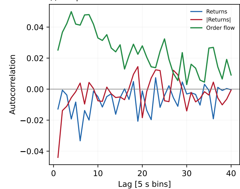
(l) Tempered ML: acf
