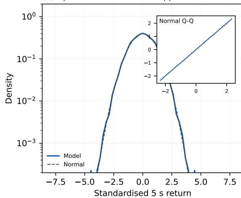
(e) Poisson: distribution qq
