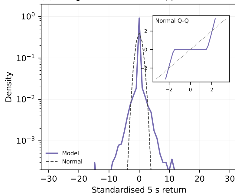
(k) Tempered ML: distribution qq
