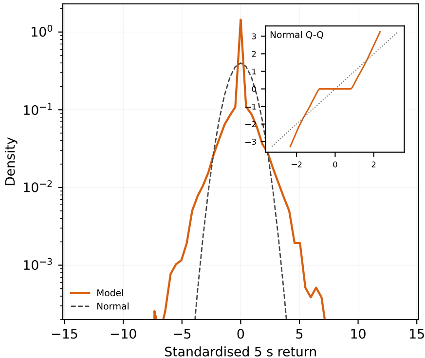
(e) Poisson: distribution qq
