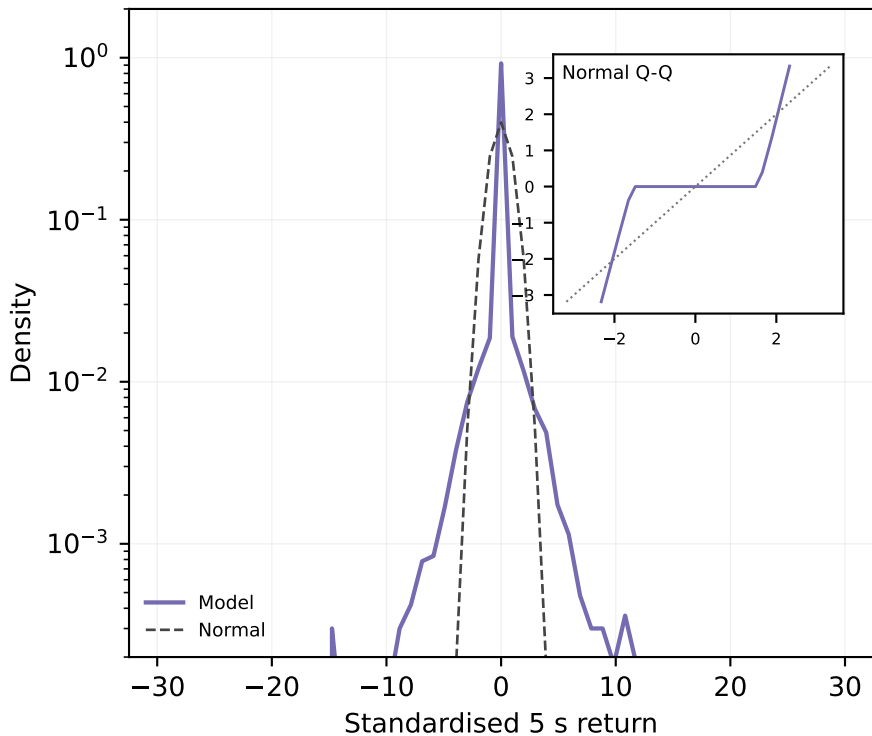
(h) Mittag-Leffler: distribution qq
