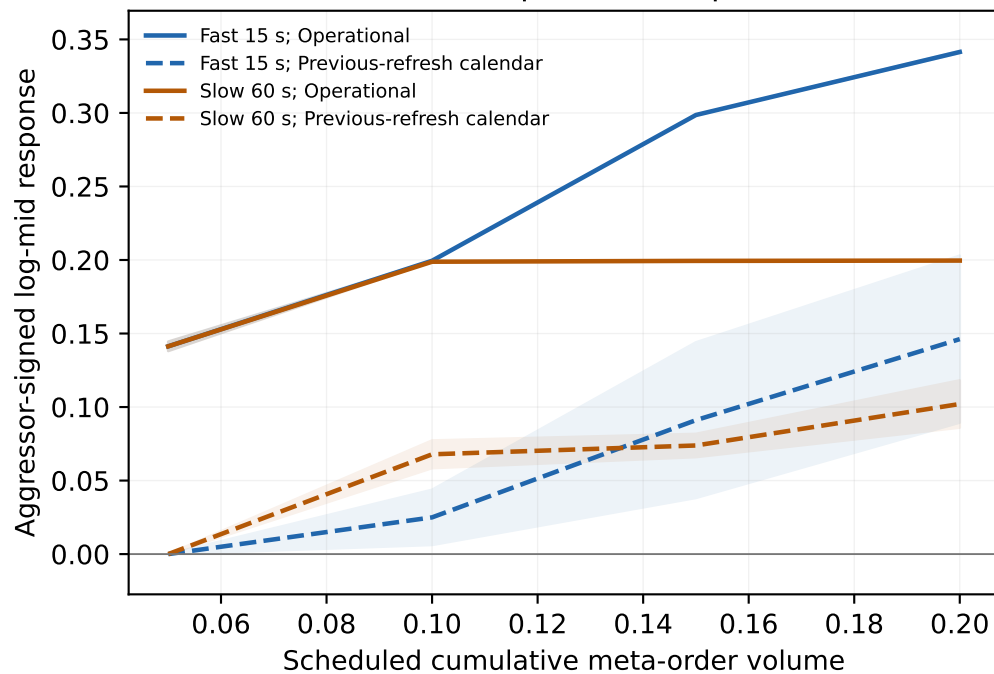
Own-impact relaxation
