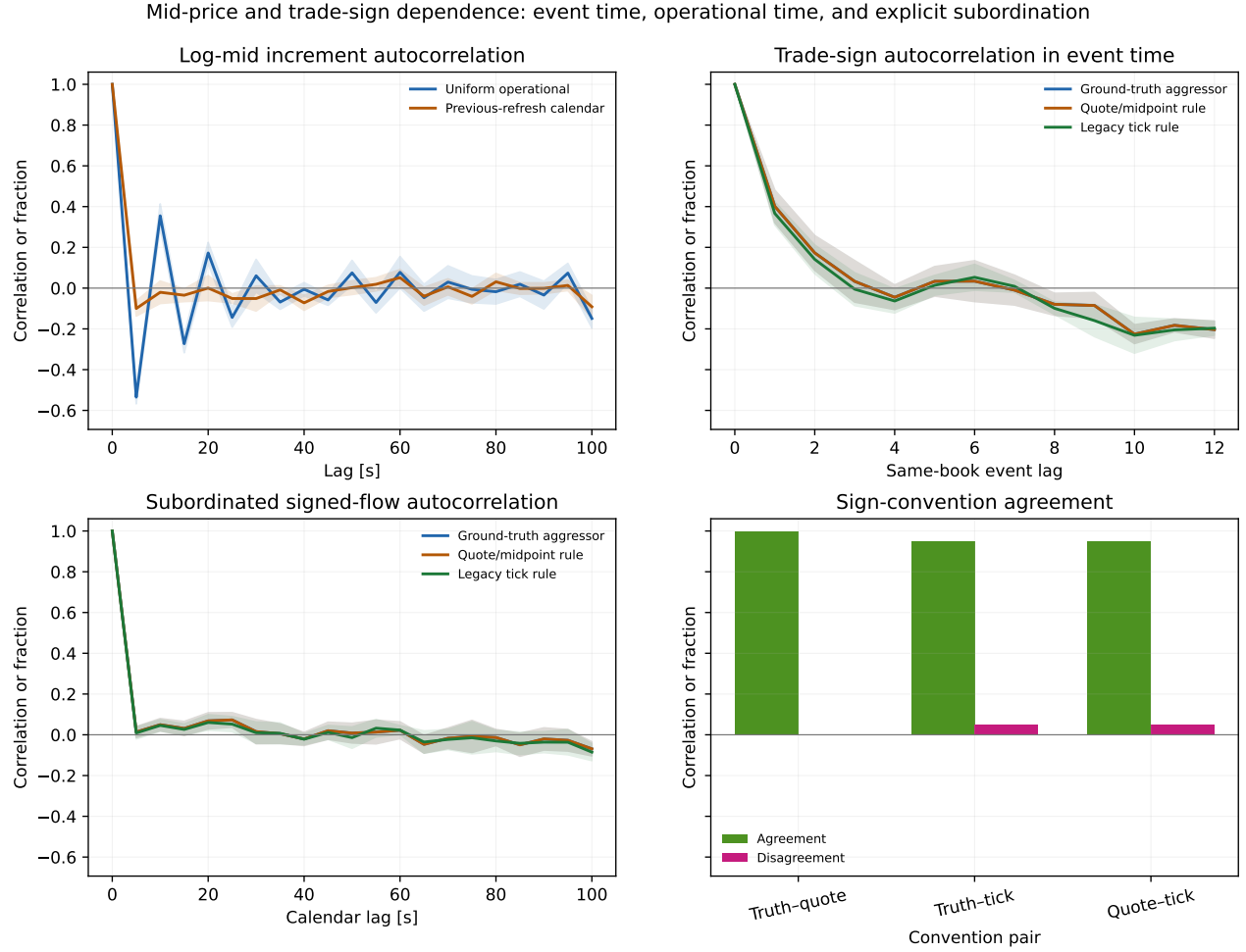
Figure 11: Mid-price and trade-sign autocorrelations. Panels report log-mid increment autocorrelation for uniform operational and previous-refresh calendar observations, same-book event-time trade-sign autocorrelation for three sign conventions, subordinated signed-flow autocorrelation, and sign-convention agreement. Price-level autocorrelation is excluded. The finite Markov persistence is an estimator fixture, not empirical calibration or an endogenous long-memory claim.
