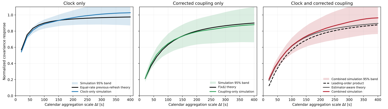
Figure 7: Final estimator-aware Epps integration. Clock-only, corrected coupling-only and combined results share one linear 0–400 second and 0–1.1 normalized-covariance scale. The combined no-refit holdout is compared with the paper’s leading-order product and the exact finite-grid, finite-step conditional moment on the same realised clocks. The estimator-aware combined RMSE is 0.039719, standardized RMSE is 0.455132, and pointwise normal-band coverage is complete. No parameter, normalization or time map is refitted.
