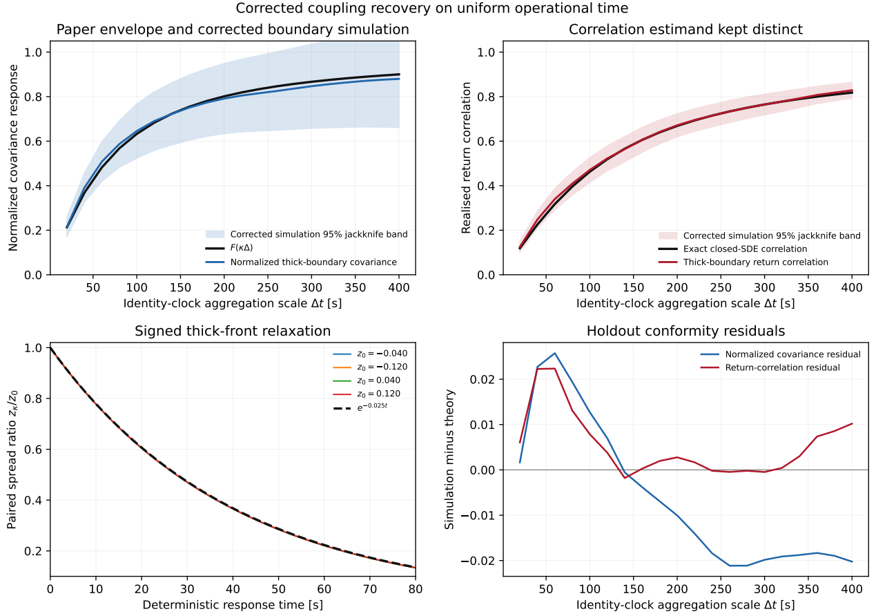
Figure 8: Corrected translation-mode coupling on uniform operational time. Holdout thick-boundary paths are compared with the analytical normalized covariance response and the distinct finite-scale return correlation. Lower panels verify signed deterministic front relaxation and residuals at the frozen response rate. No clock, interpolation or parameter fit enters this component gate.
