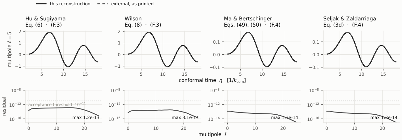
F1 The covariant free-streaming recursion against four external hierarchies
